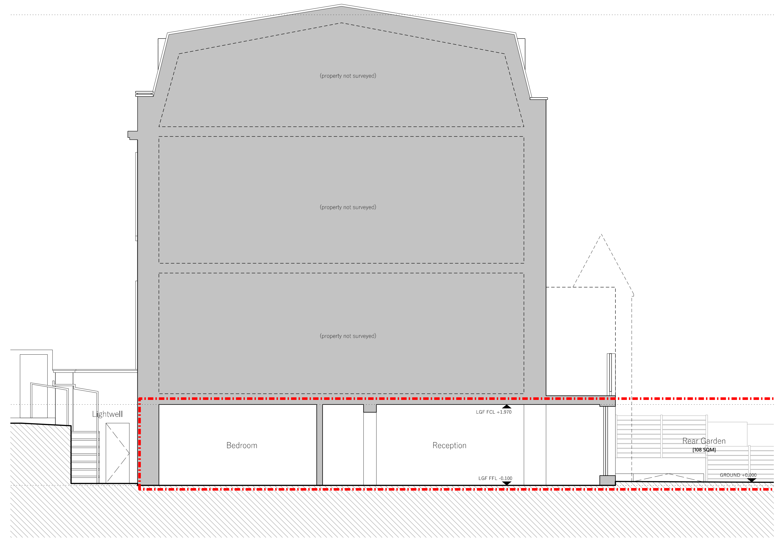
Existing Section
