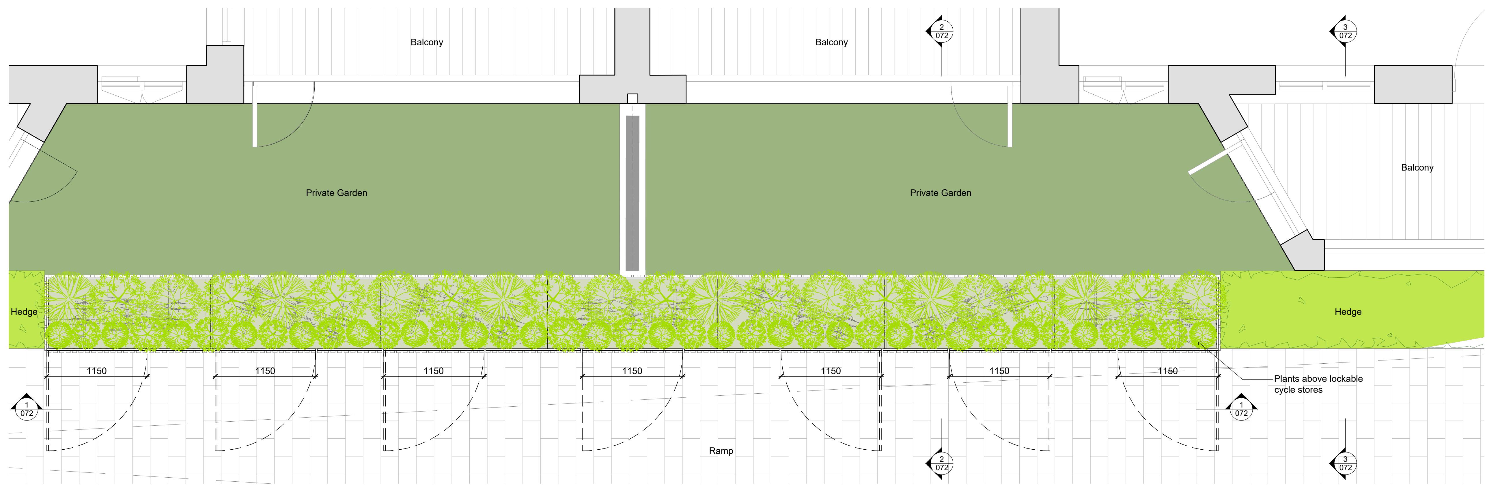
1B 071 Building C - Planter above Cycle Storage Plan
