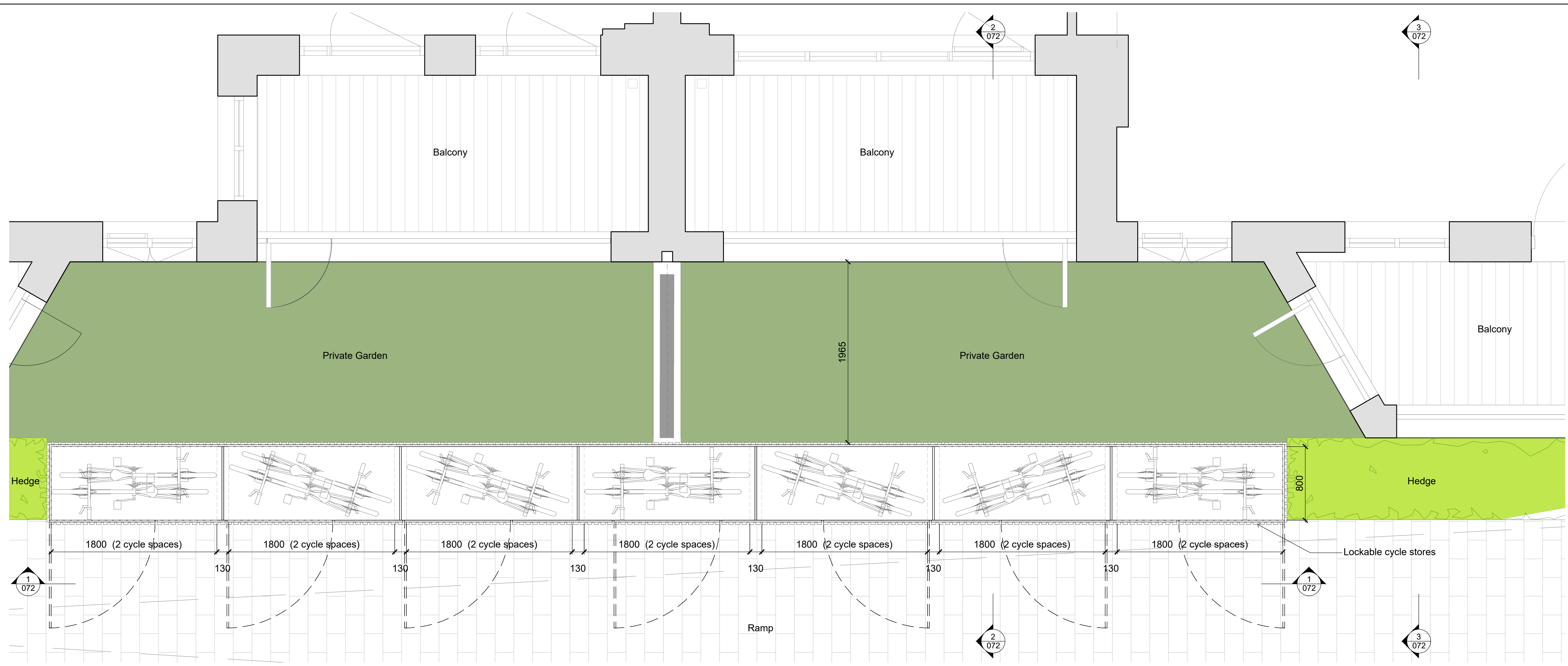
1A 071 Building C - Cycle Storage Plan
