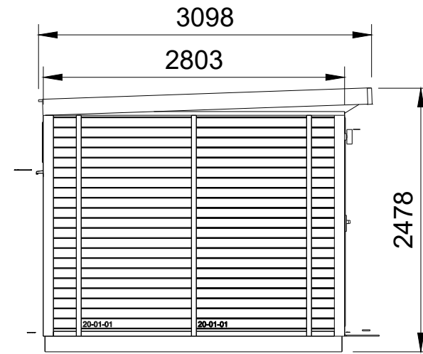
Left Elevation
