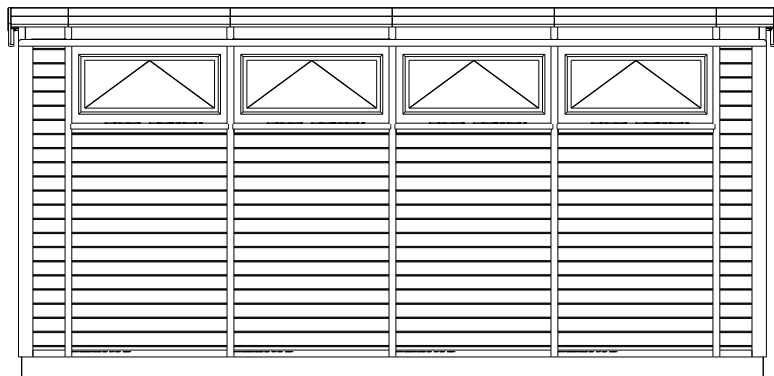
Rear Elevation
