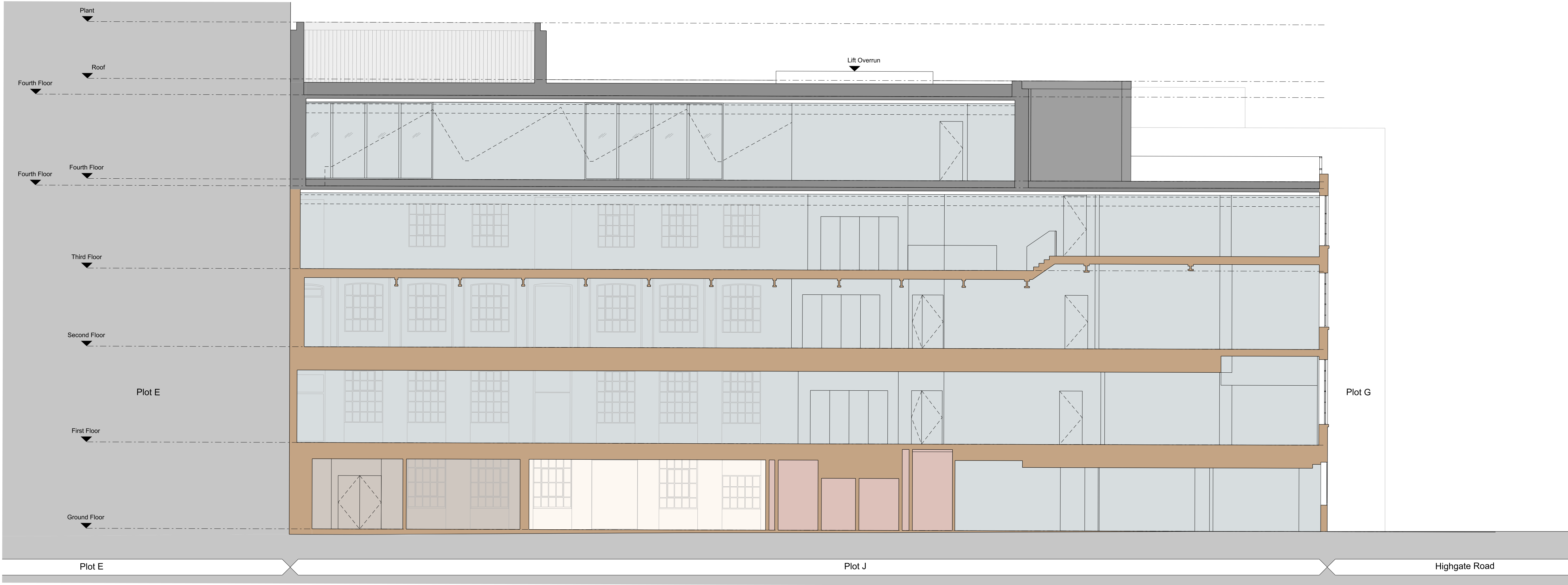
2 PLOT J SECTION BB SCALE 1:100
