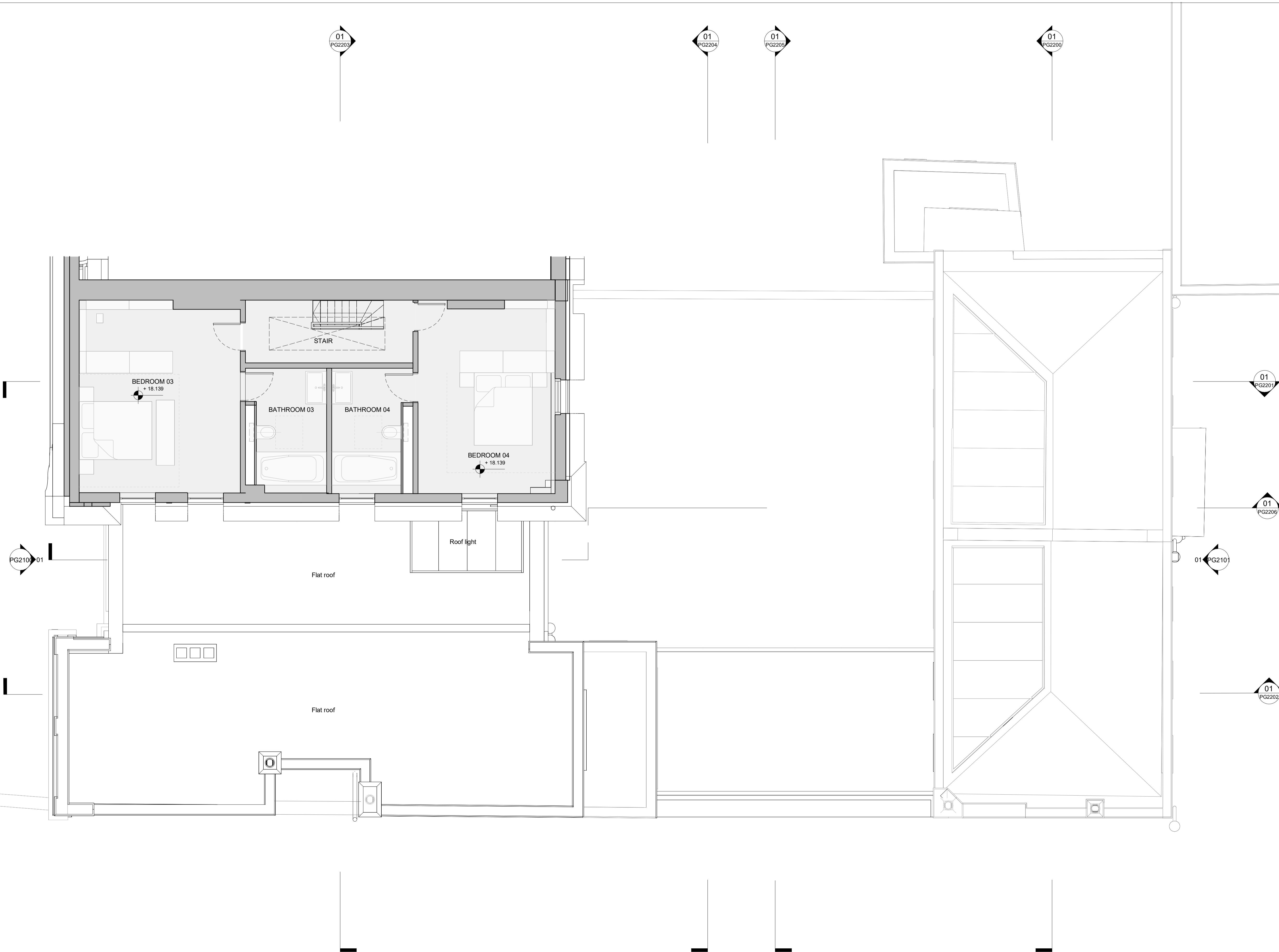
01 Consented Second Floor Plan 1 : 50
