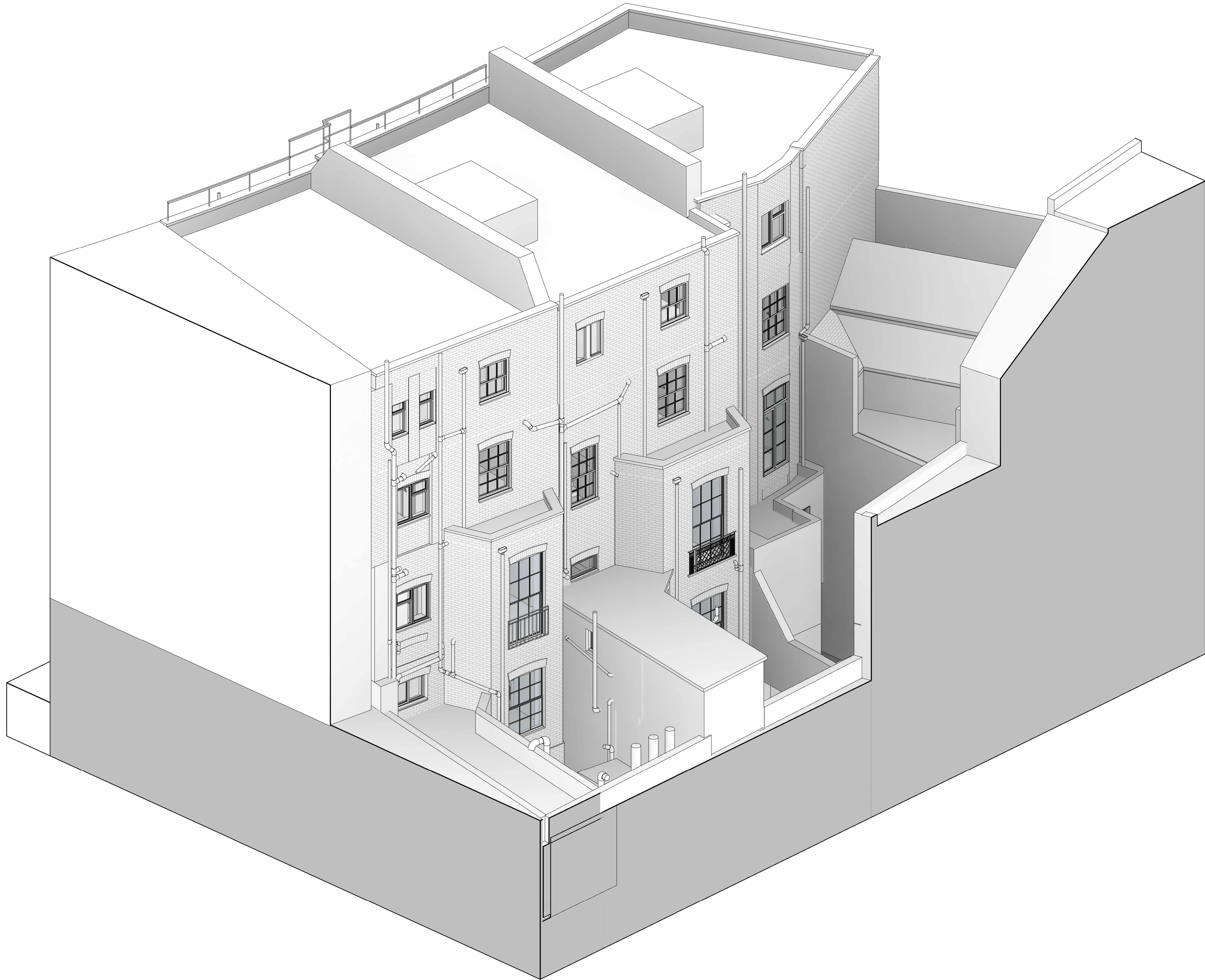
1 Existing Isometric View 2
