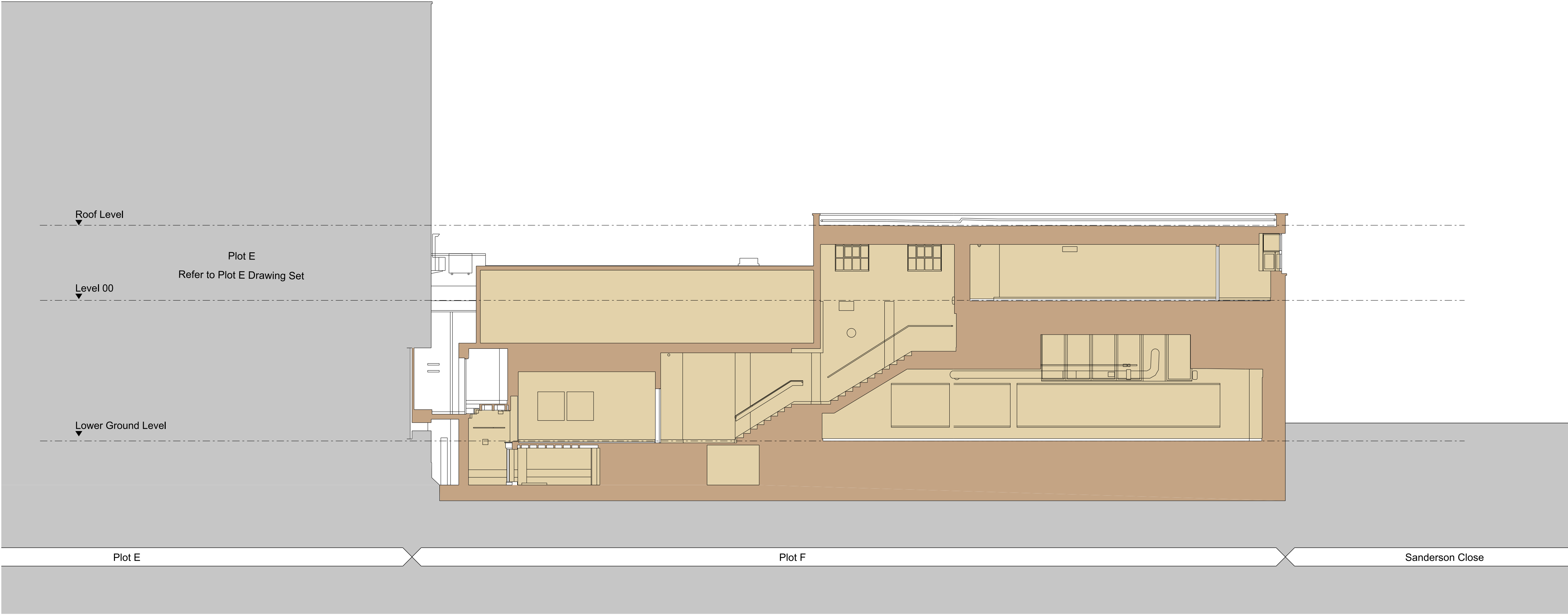
2 PLOT F SECTION BB SCALE 1:100
