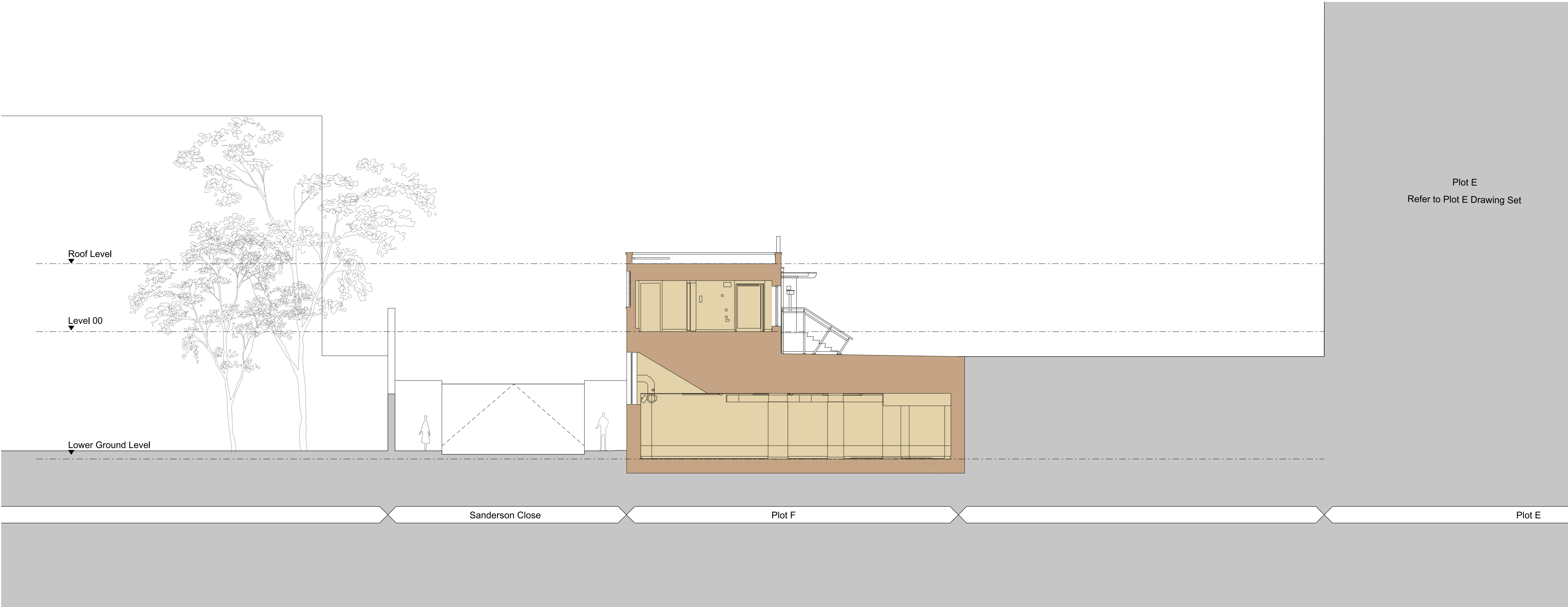
1 PLOT F SECTION AA SCALE 1:100
