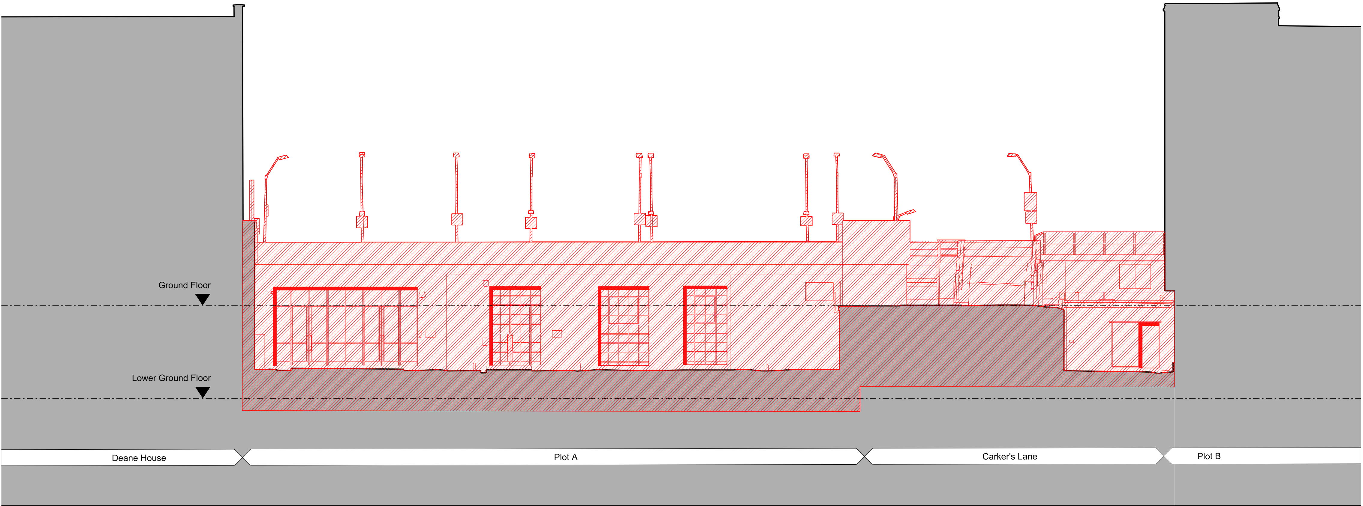
2 PLOT A ELEVATION SCALE 1:100
