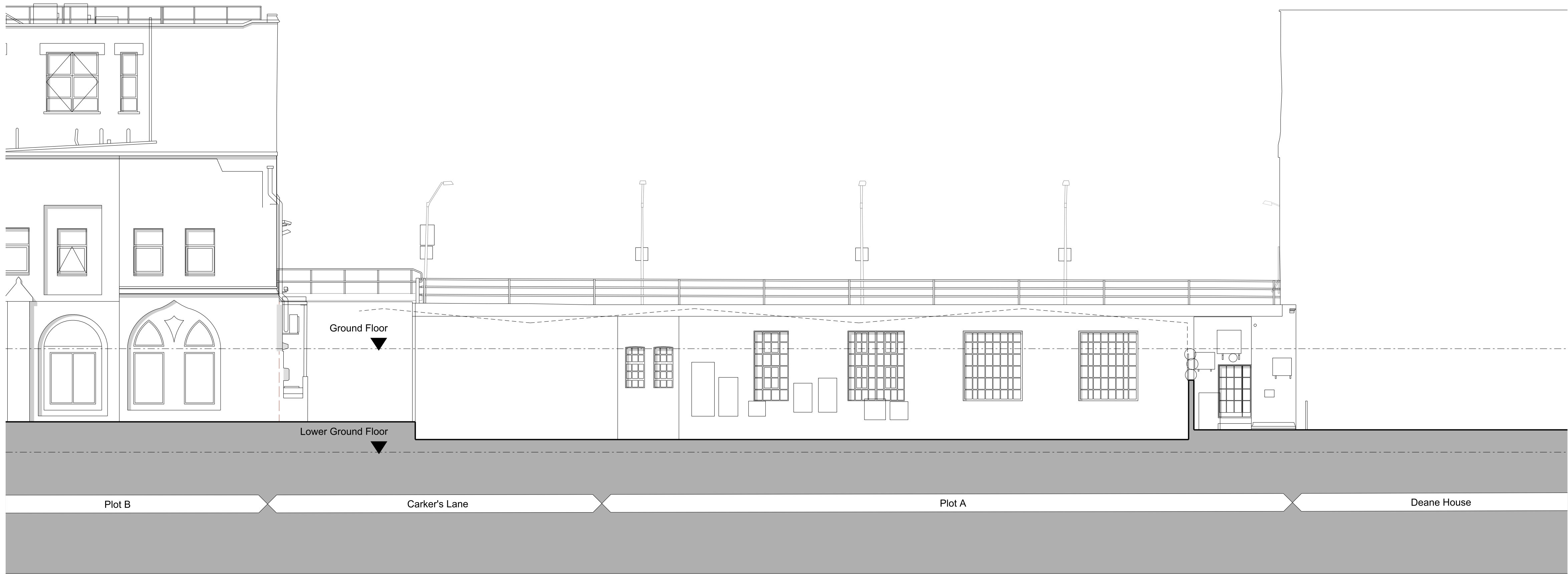
1 PLOT A ELEVATION SCALE 1:100
