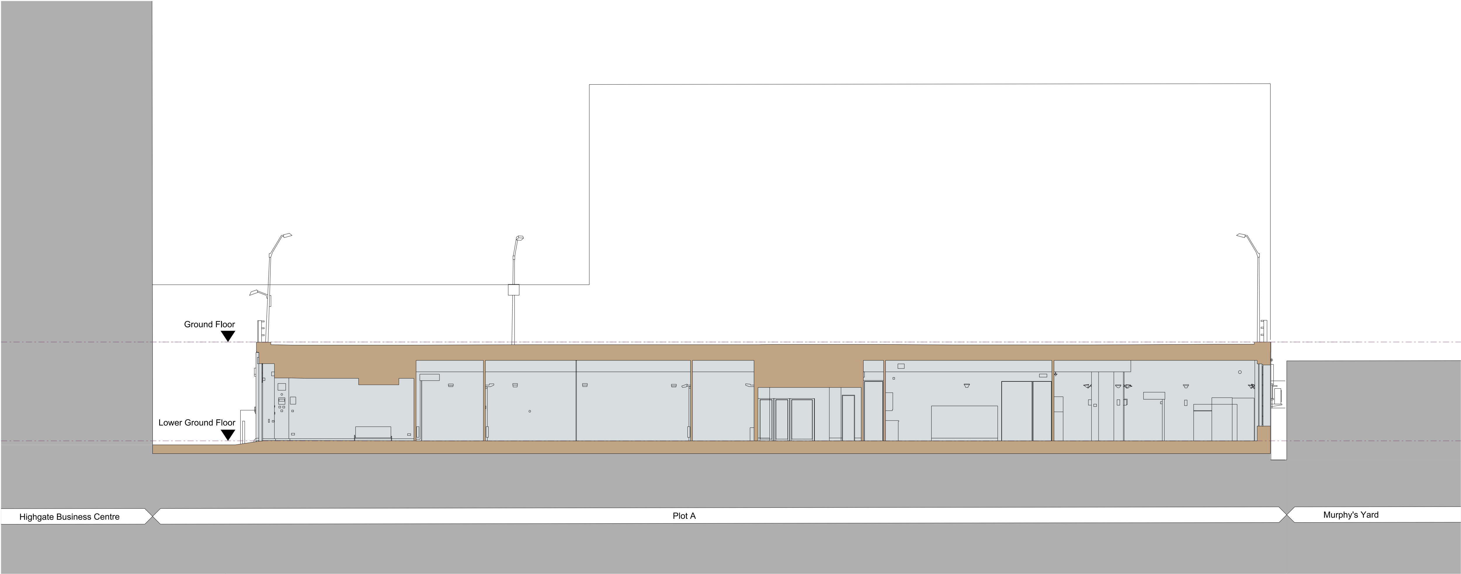
2 PLOT A EXISTING SECTION BB SCALE 1:100
