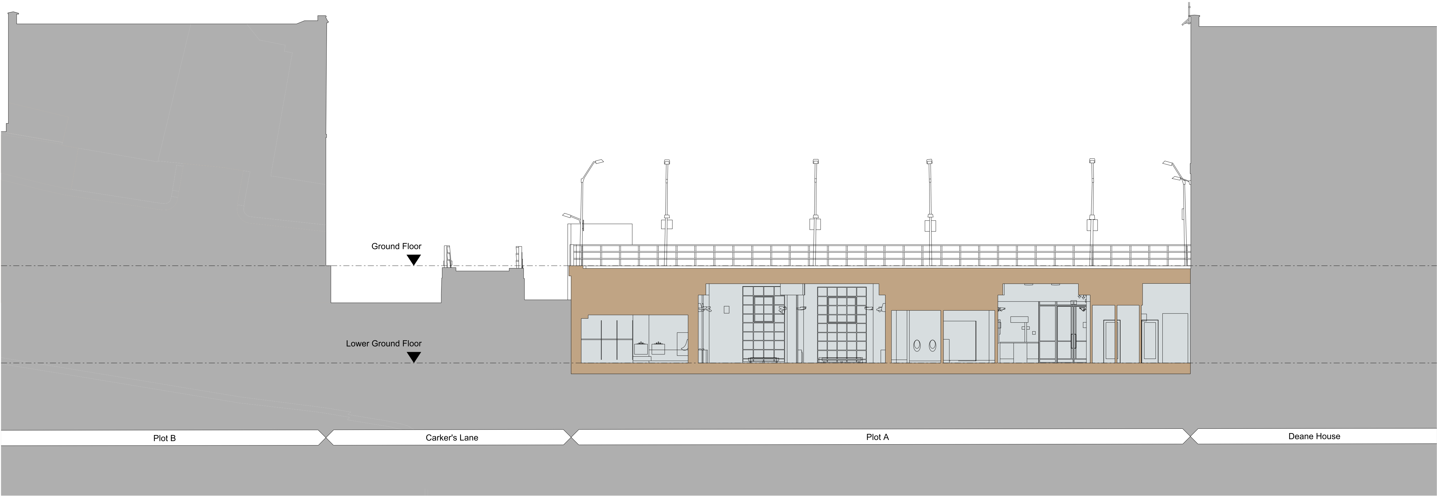
1 PLOT A EXISTING SECTION AA SCALE 1:100
