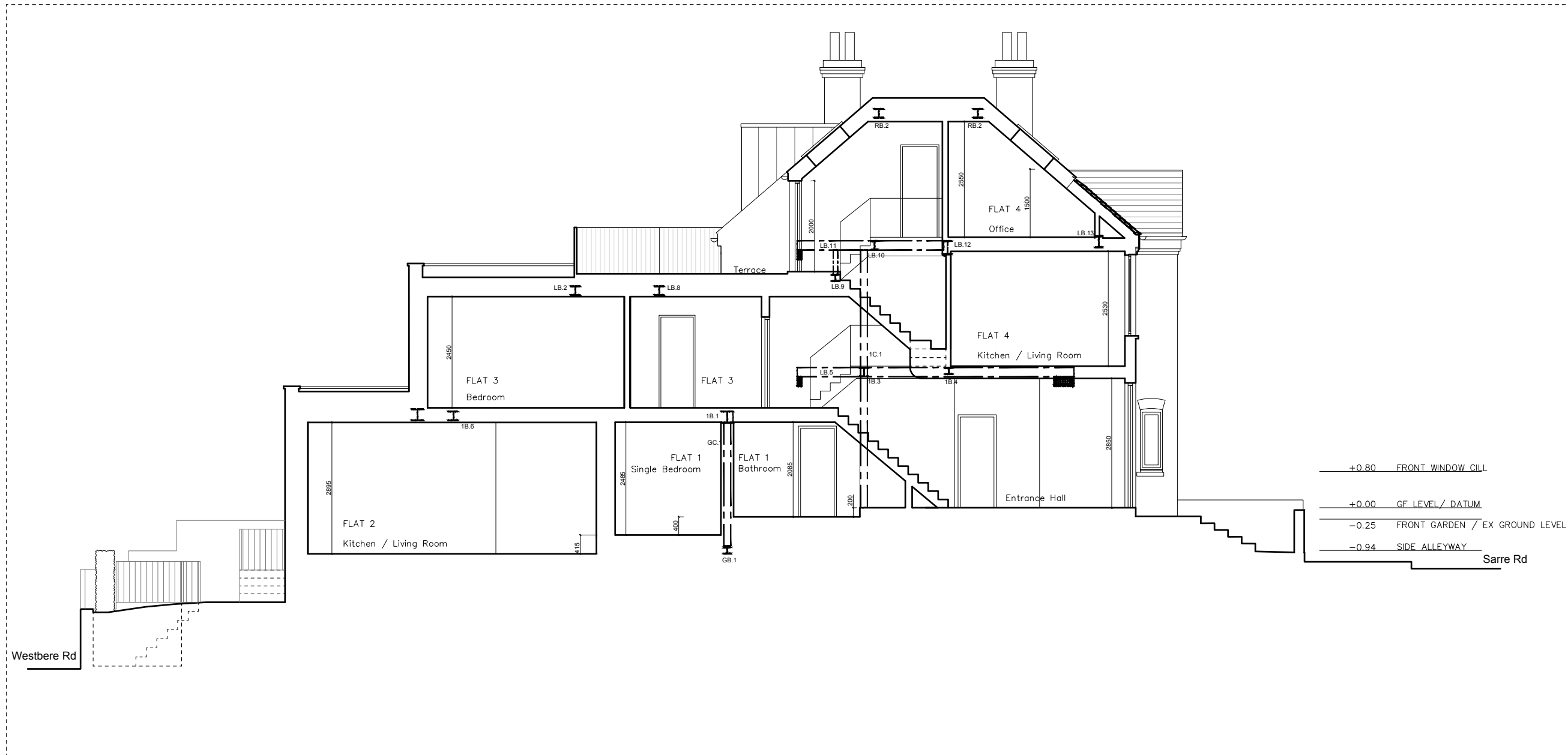
SECTION B-B'
