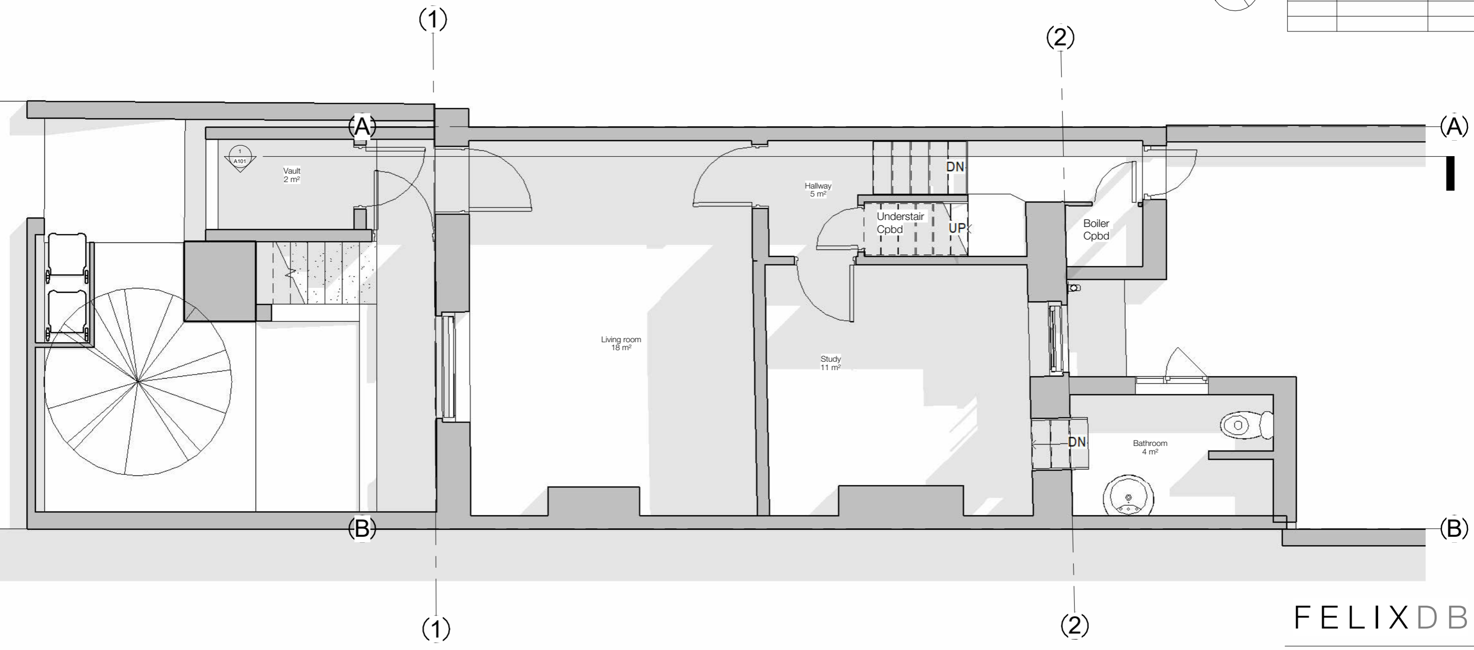
1 -1 Lower Ground Floor - Existing 1.50 1 : 50
