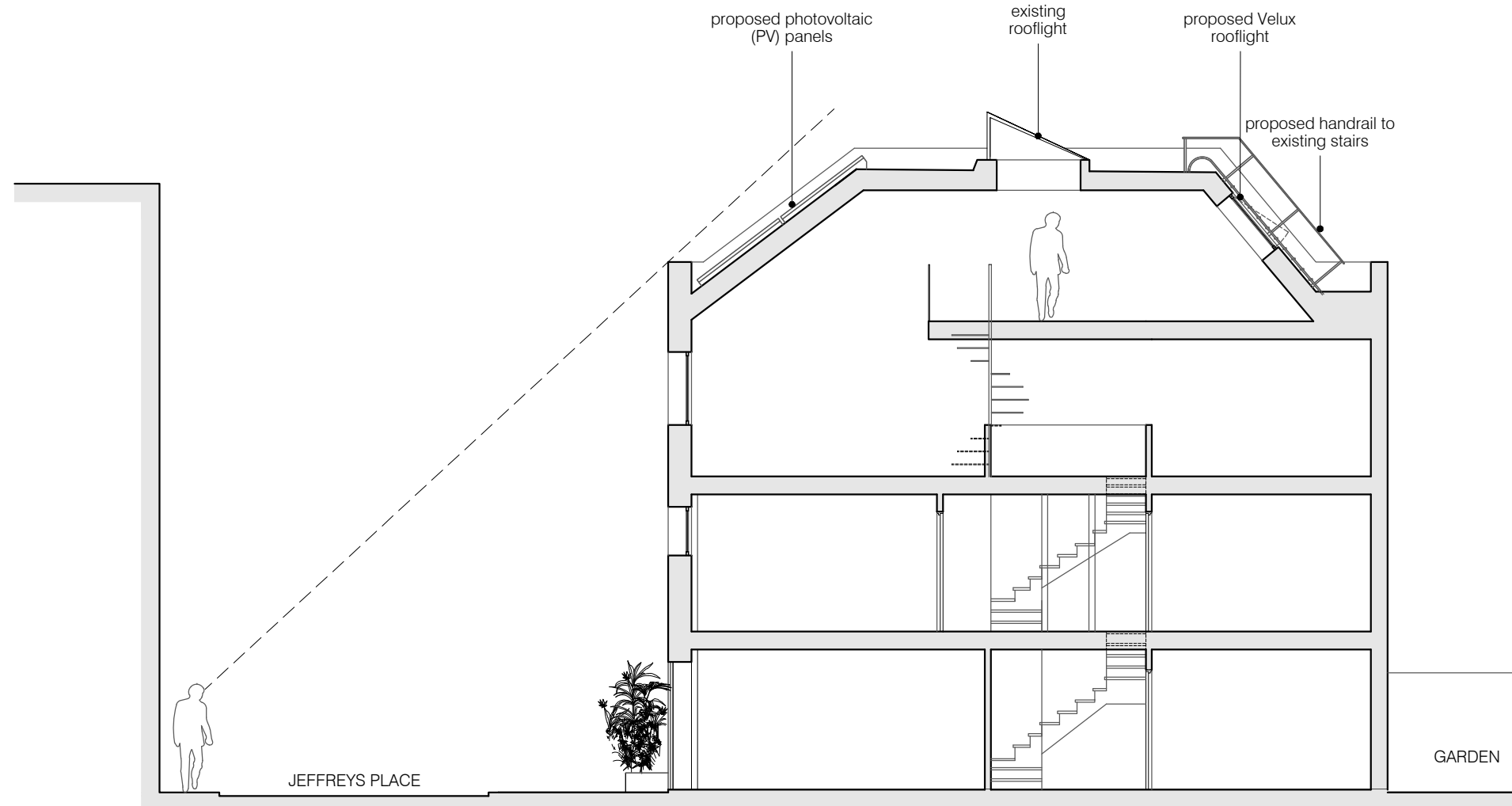
01 PROPOSED EXTENDED SECTION A-A scale 1:100
