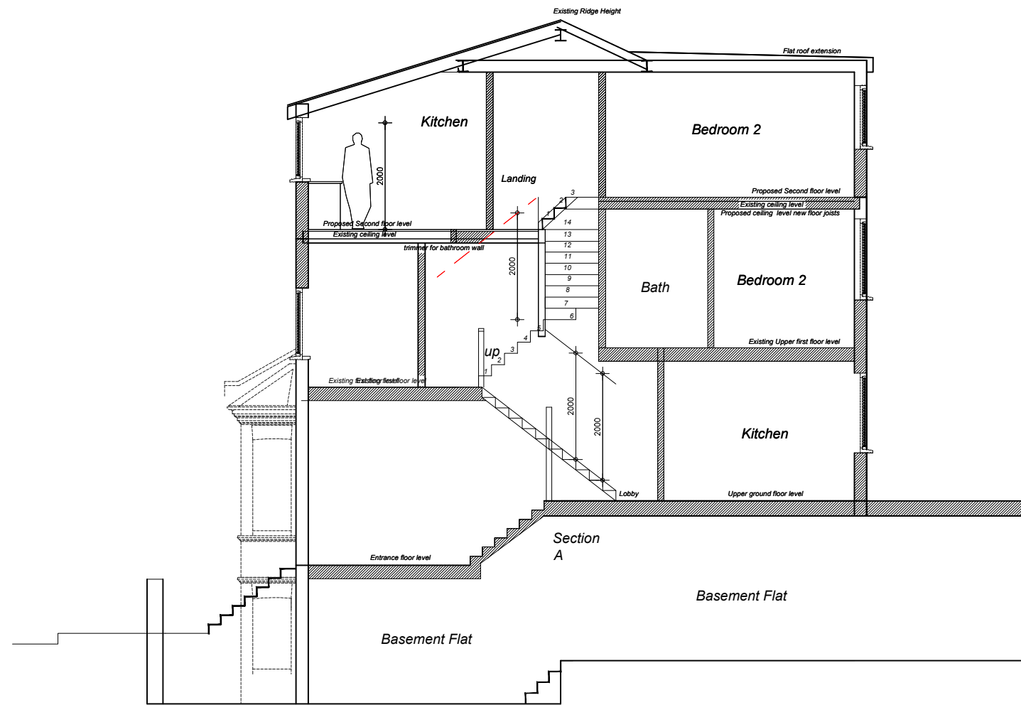
Proposed Section
