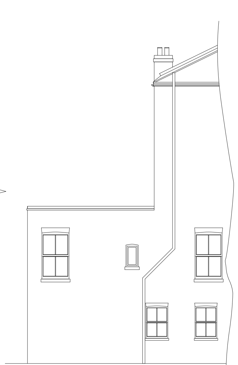
Elevation CC
