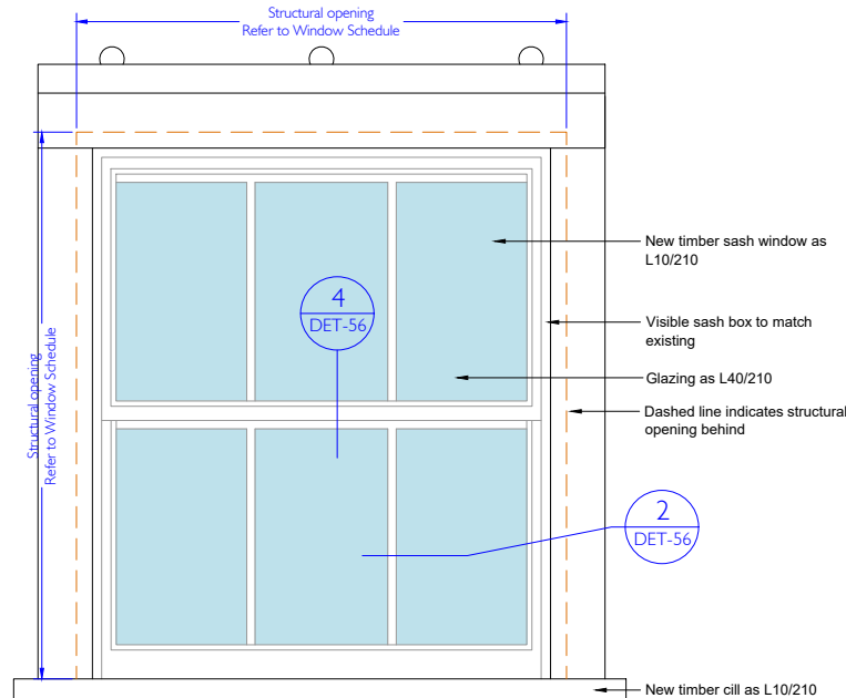
4 NEW SASH WINDOW TYPE 4 - ELEVATION
