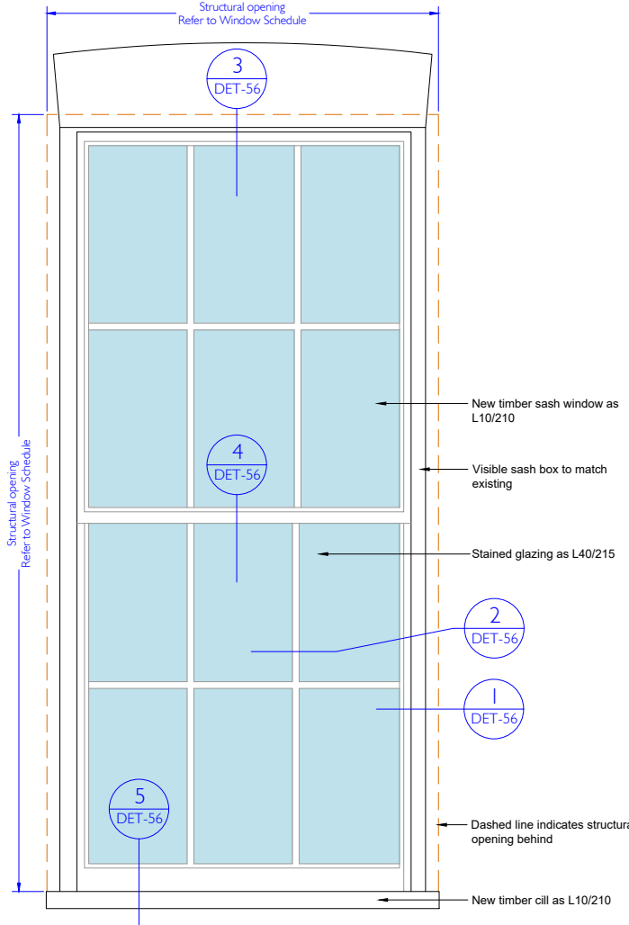
2 NEW SASH WINDOW TYPE 2 - ELEVATION
