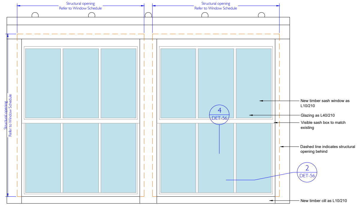
3 NEW SASH WINDOW TYPE 3 - ELEVATION
