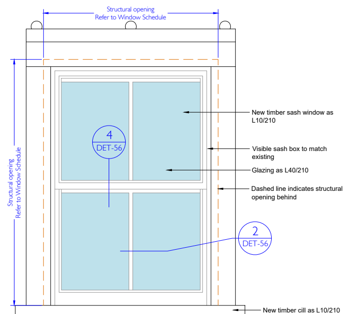
5 NEW SASH WINDOW TYPE 5 - ELEVATION
