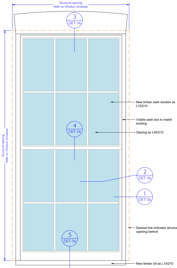
1 NEW SASH WINDOW TYPE 1 - ELEVATION
