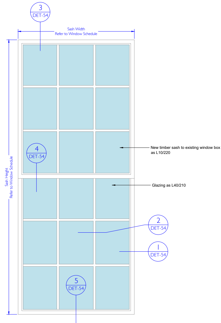
2 DET-53 REPLACEMENT SASH TYPE 2 - ELEVATION
