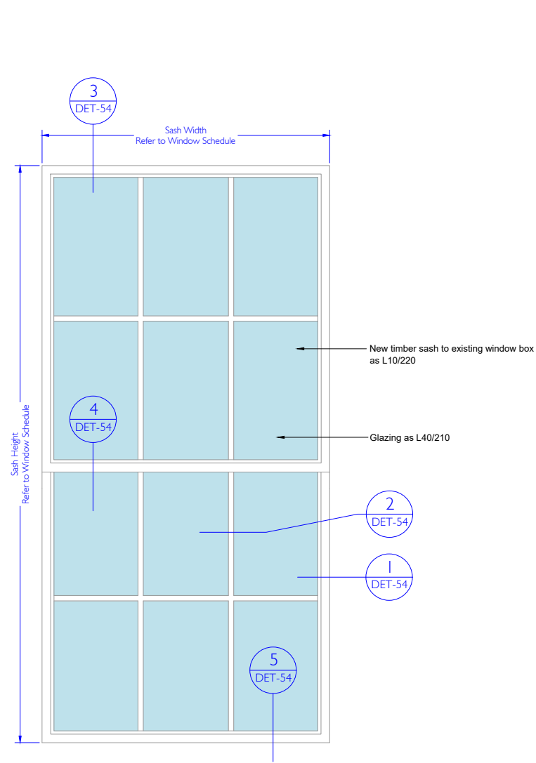
1 DET-53 REPLACEMENT SASH TYPE 1 - ELEVATION
