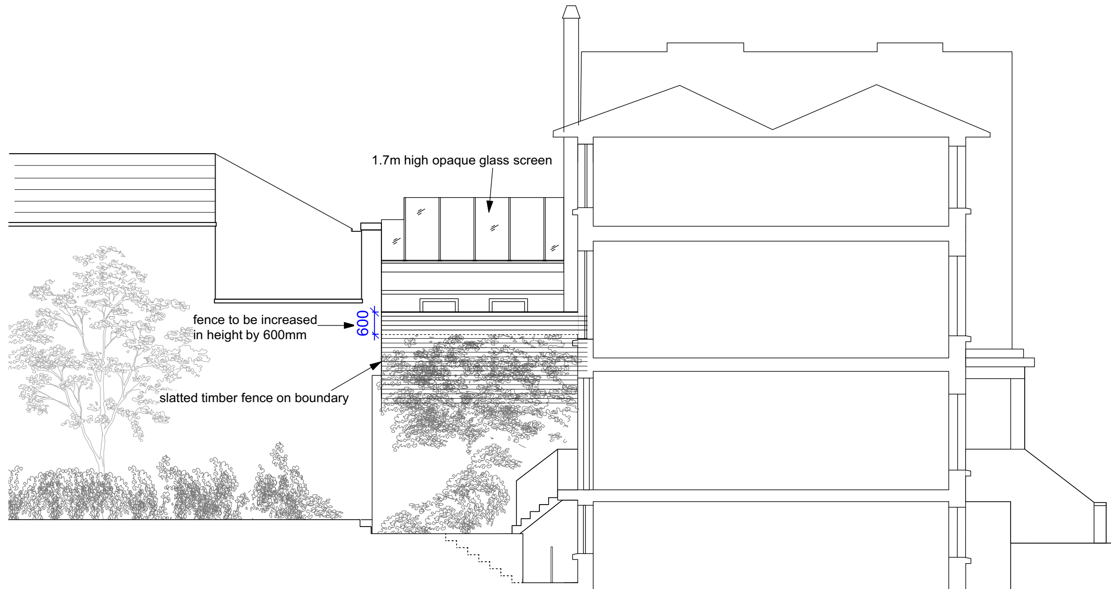
Section through 71 Haverstock Hill
