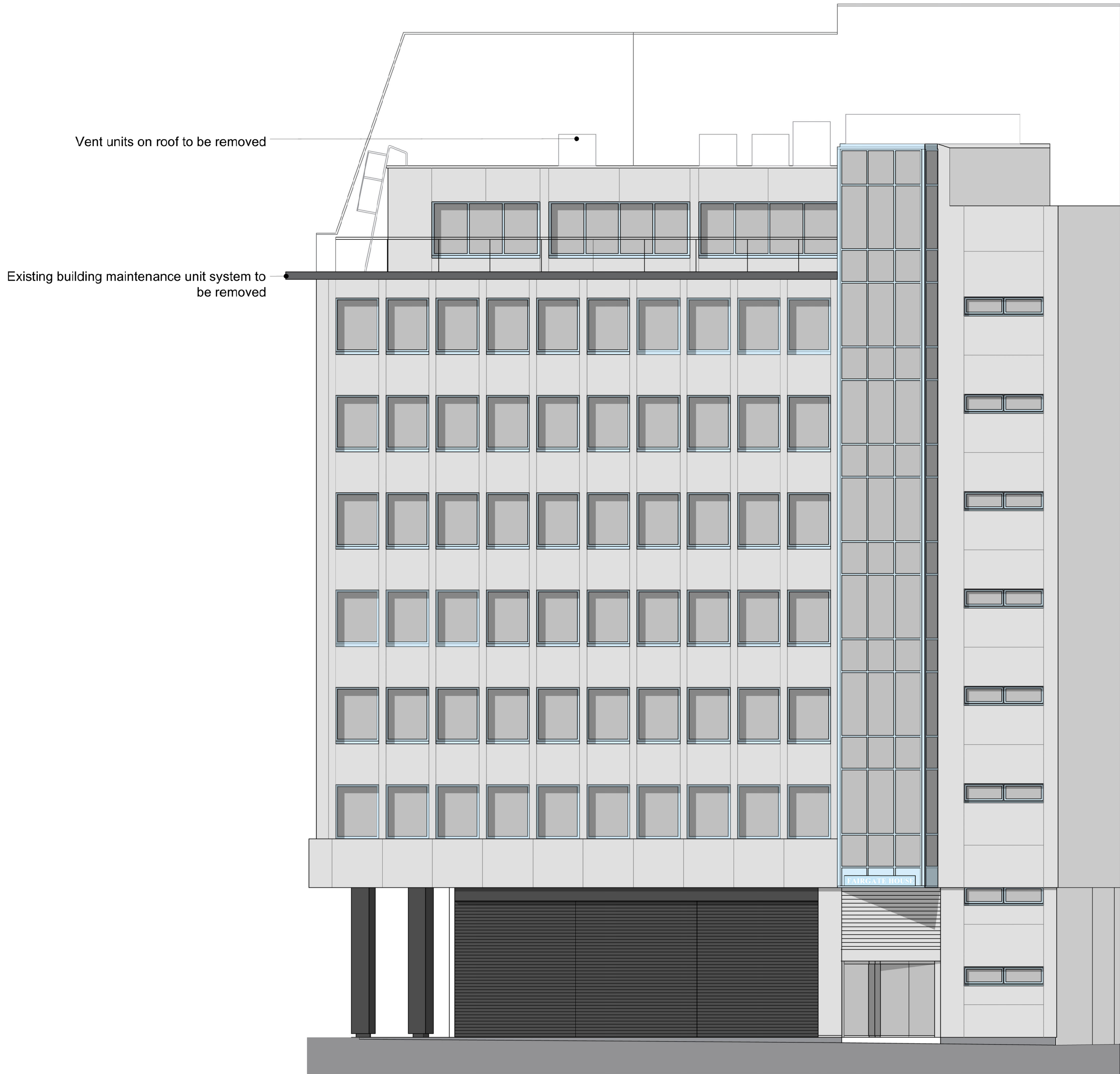
1 Existing Dyott Street Elevation 1 : 100
