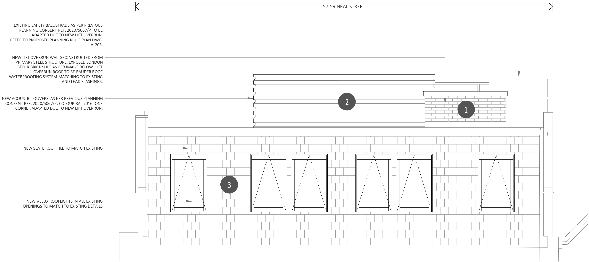
(A) Detail elevation of lift overrun and acoustic enclosure.
