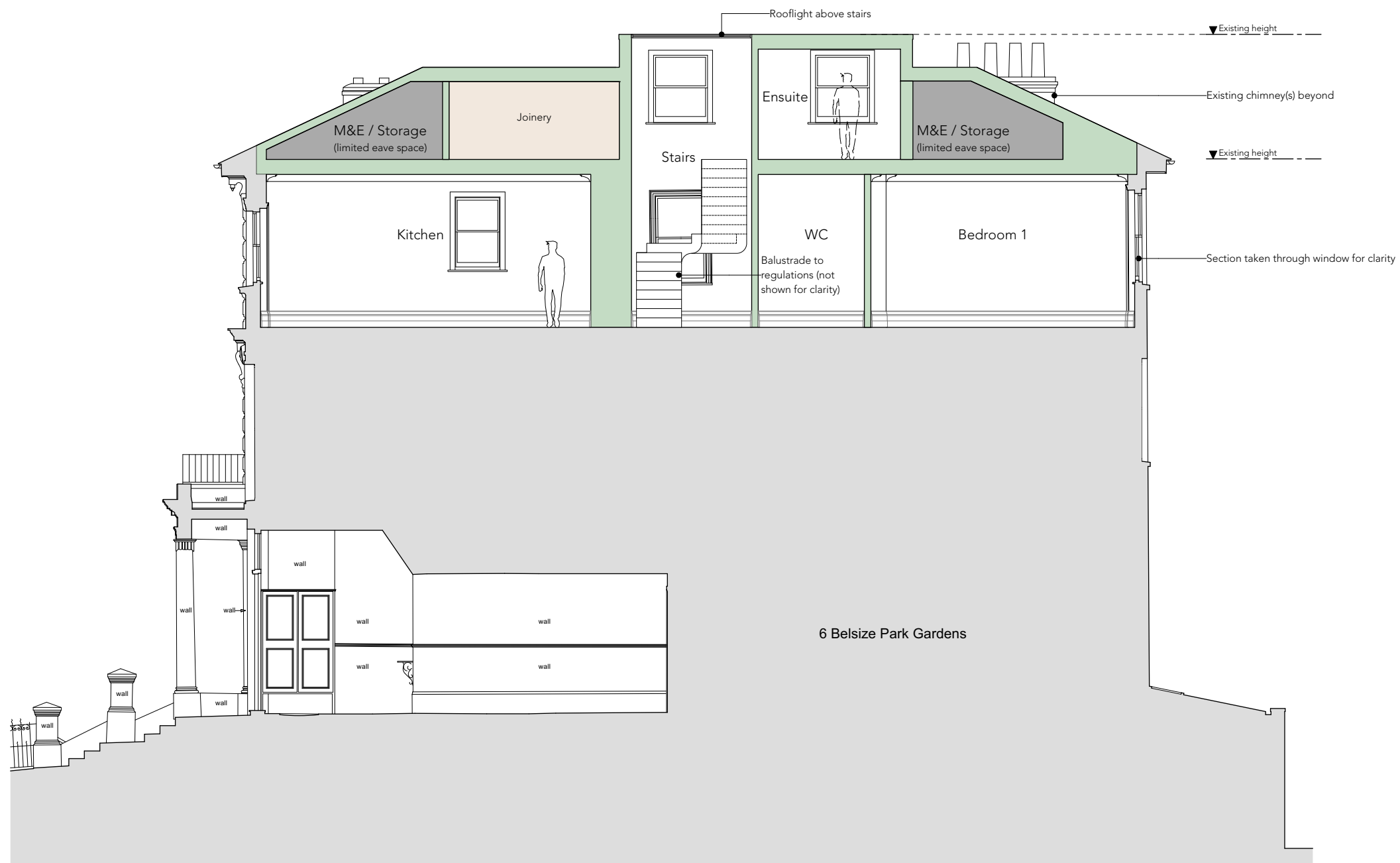
1 Proposed Section 4 Scale: 1:100 @ A3
