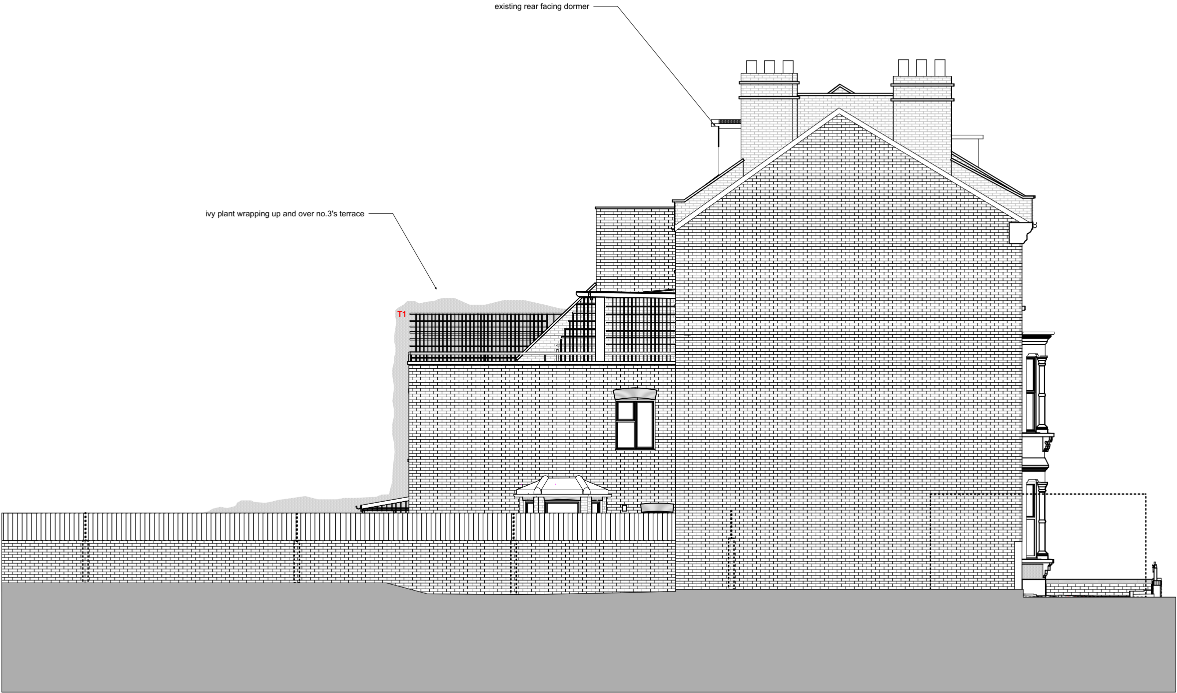
South Elevation
