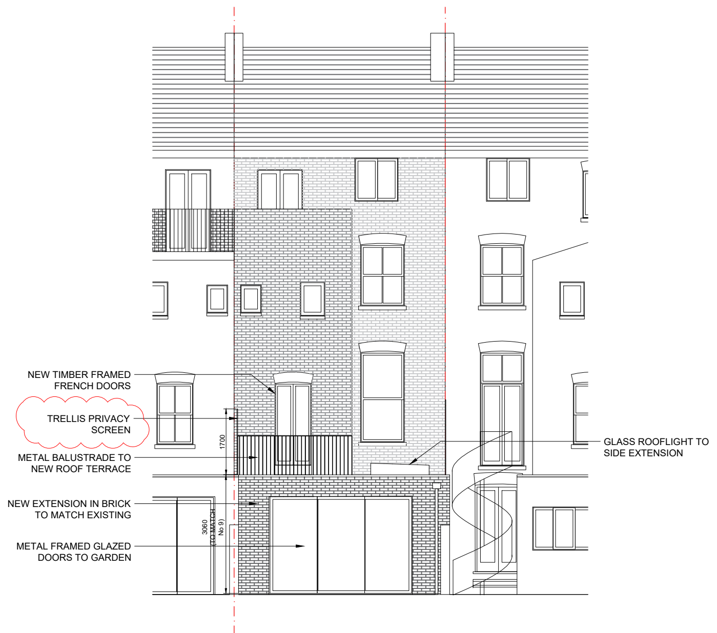
pAA PROPOSED ELEVATION AA 0 0.5 1 2 3 1:50 at A1
