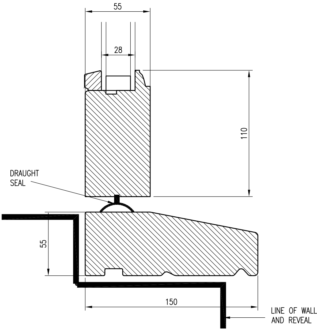
CILL SECTION SCALE 1:2
