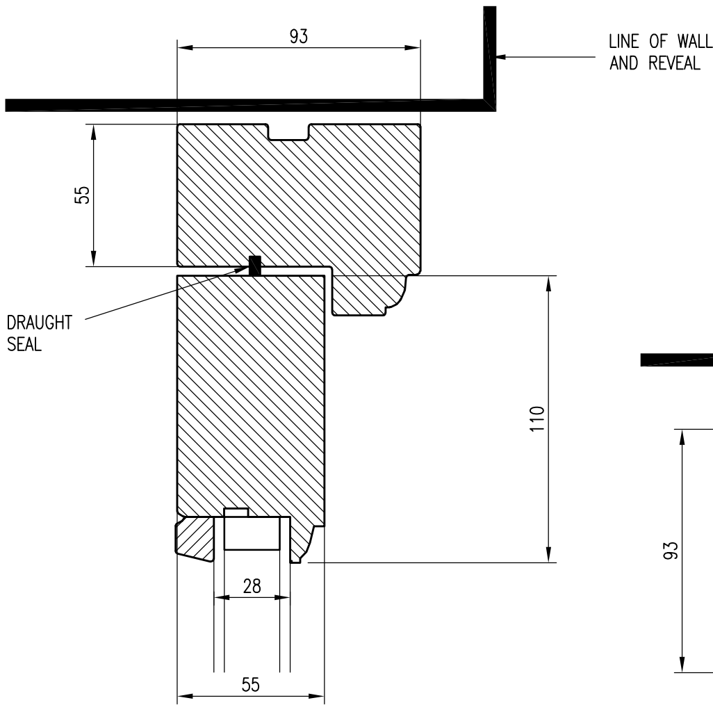
HEAD SECTION SCALE 1:2
