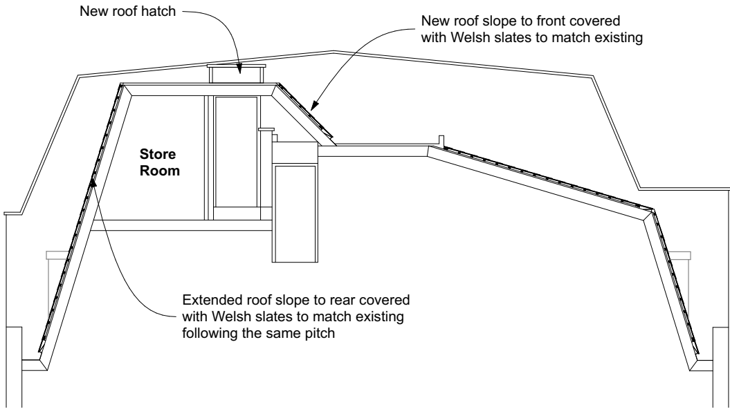
Proposed Roof Section - S01
