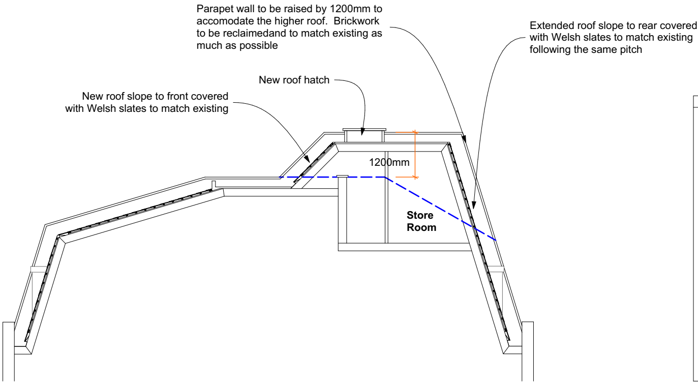
Proposed Roof Section - S02
