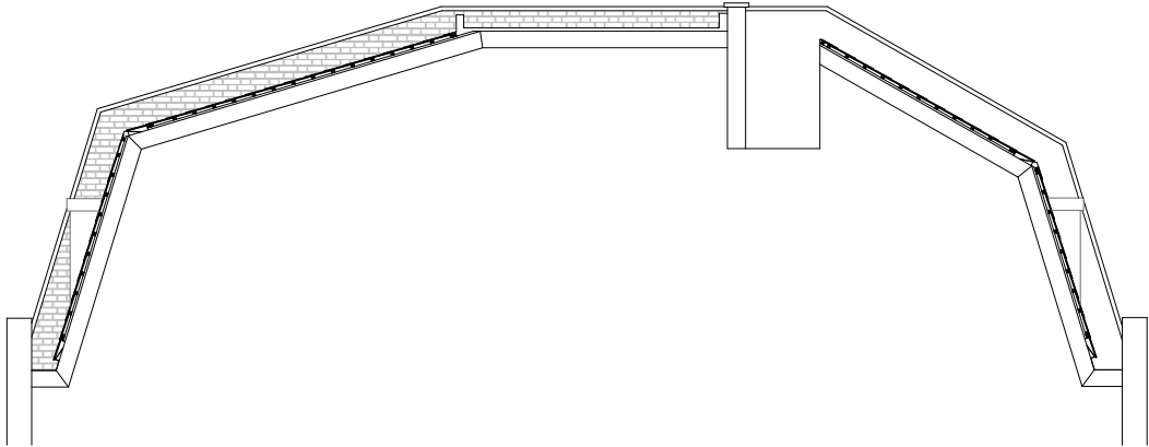
Existing Roof Section - S02
