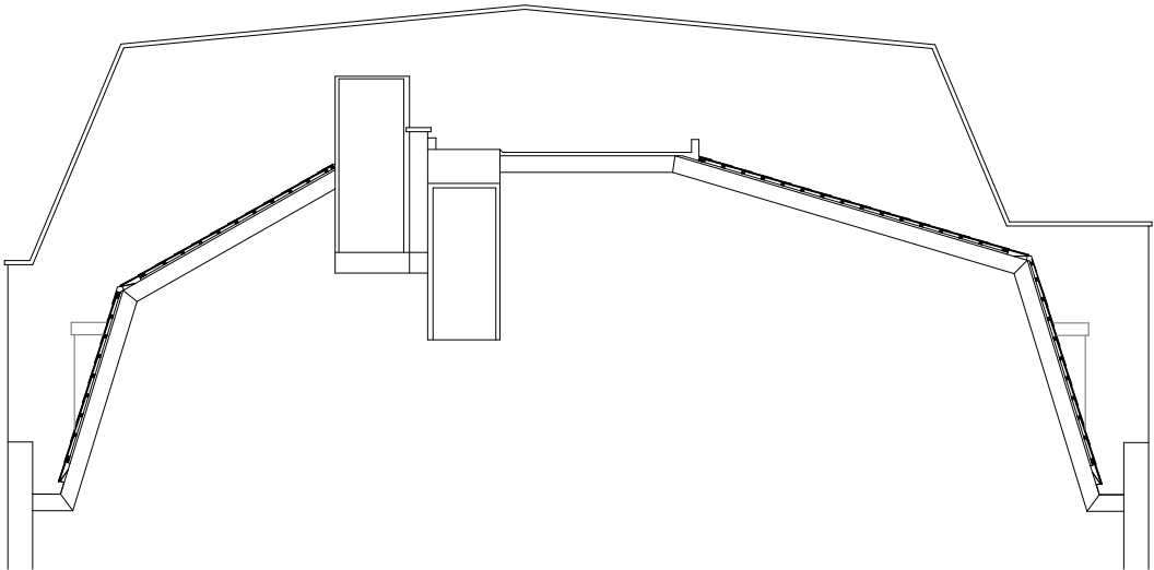
Existing Roof Section - S01
