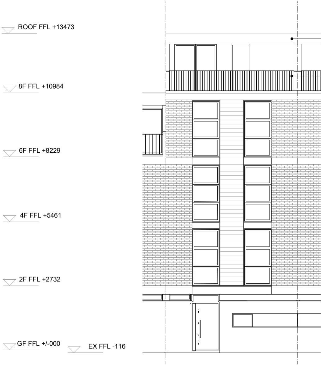
(01)250.01 Front Elevation
