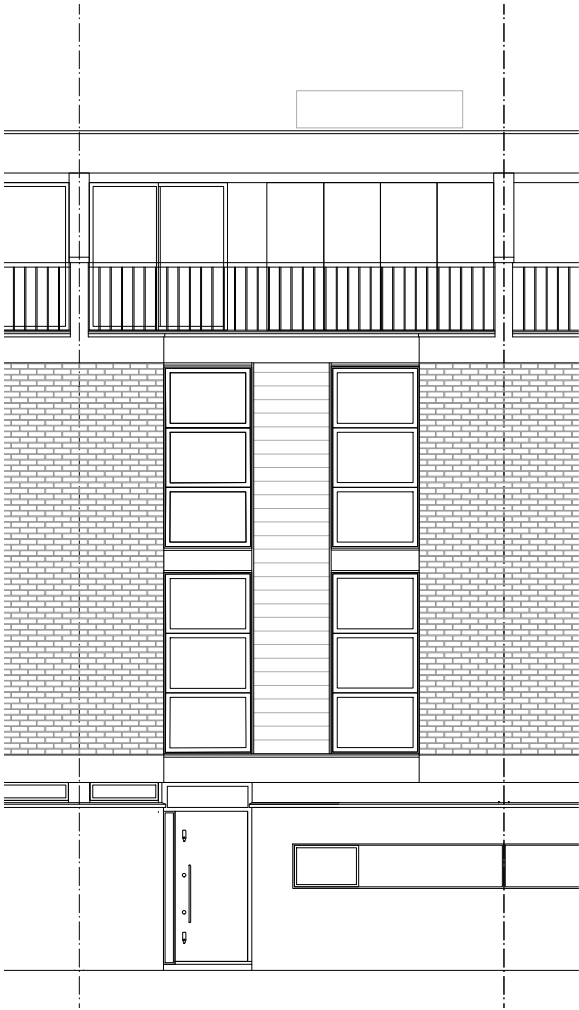
(00)250.01 Front Elevation
