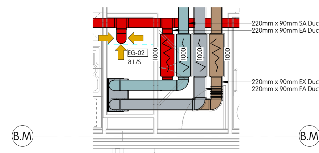
AI 2B4P_A TYPE 1_B Handed version
