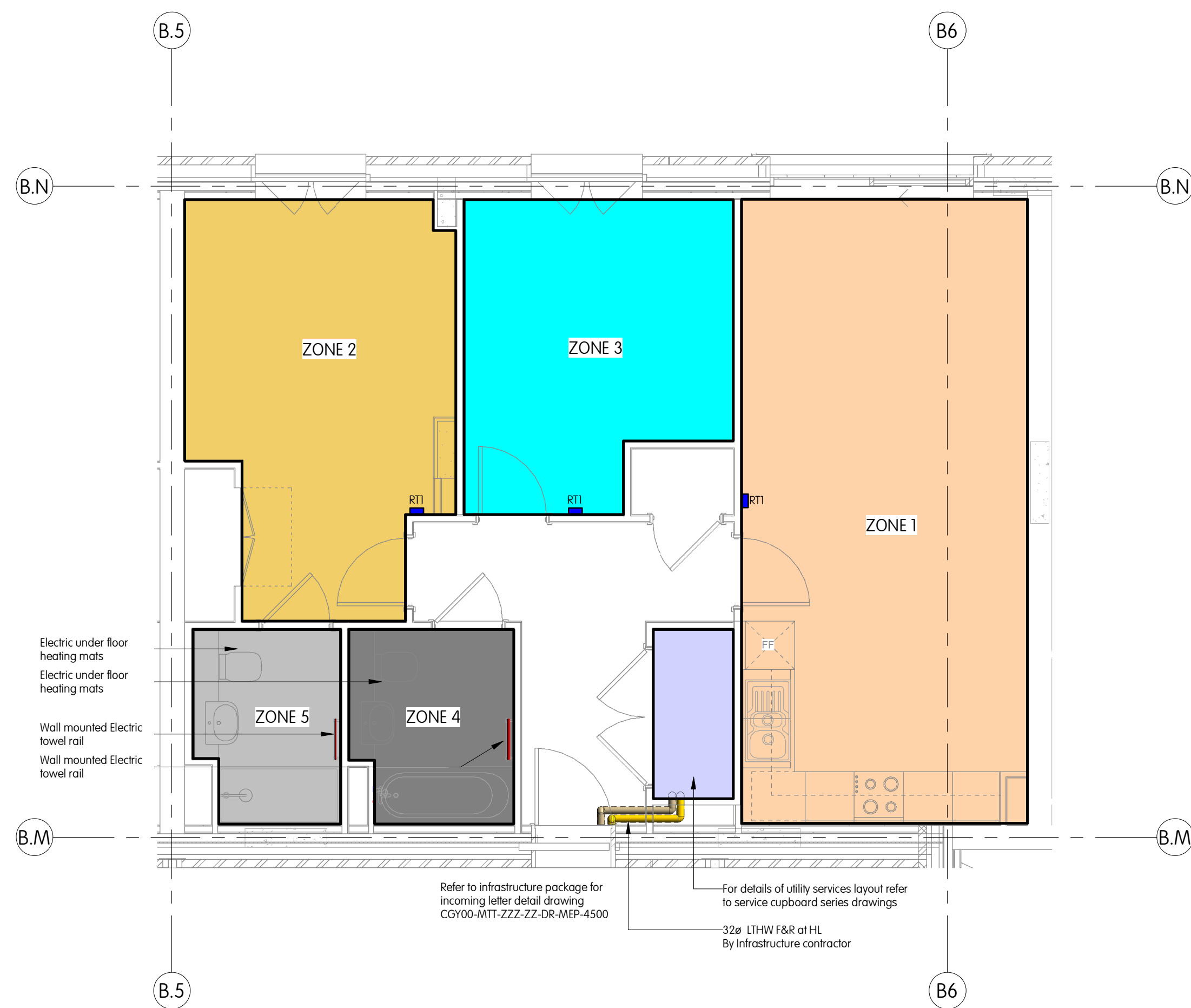
AI 2B4P_A TYPE 1_B Heating Layout
