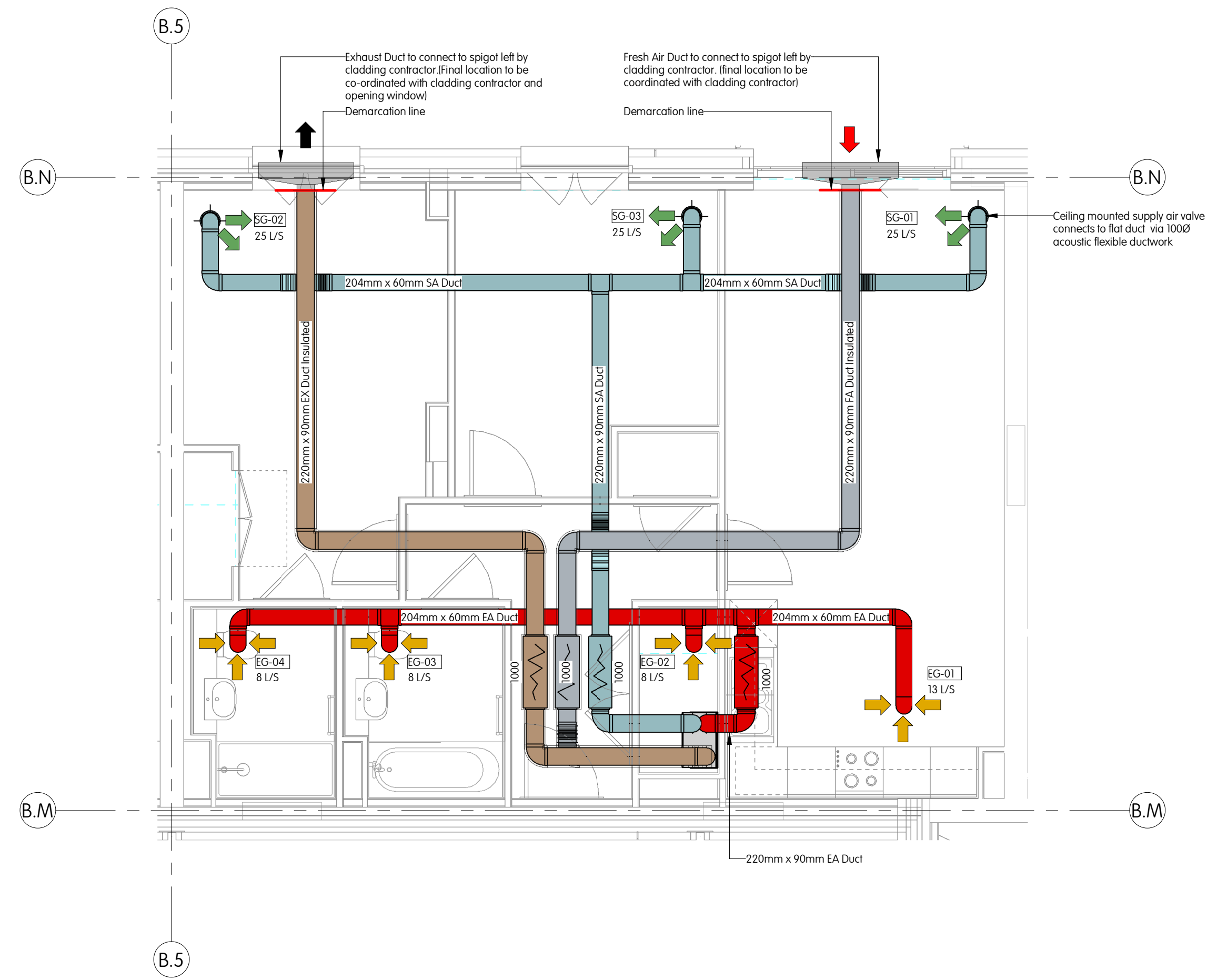
AI 2B4P_A TYPE 1_B Ventilation
