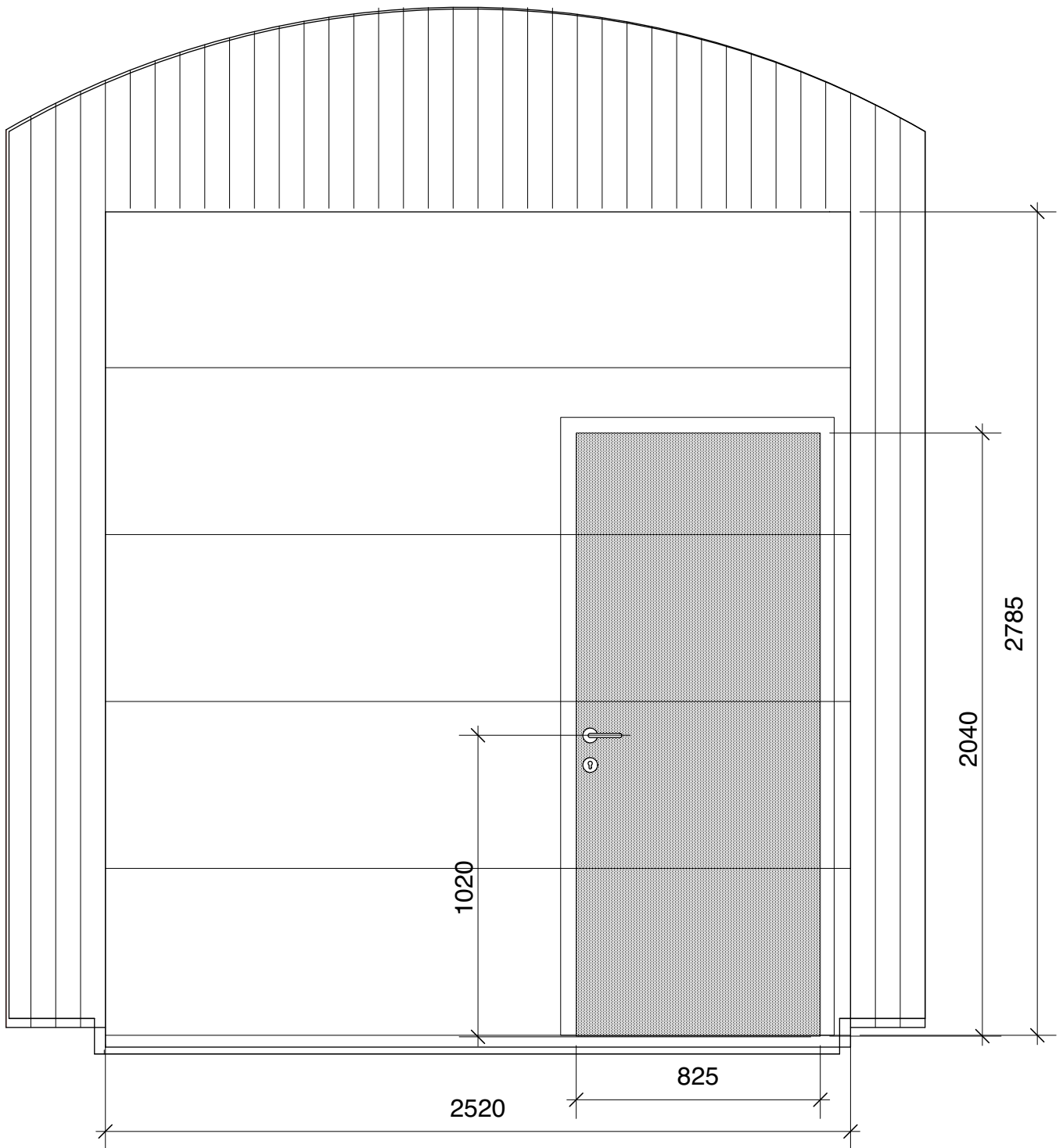
32 Coptic Street Garage door with Wicket Door for Antony Peattie Esq External Street Elevation to Coptic Street
