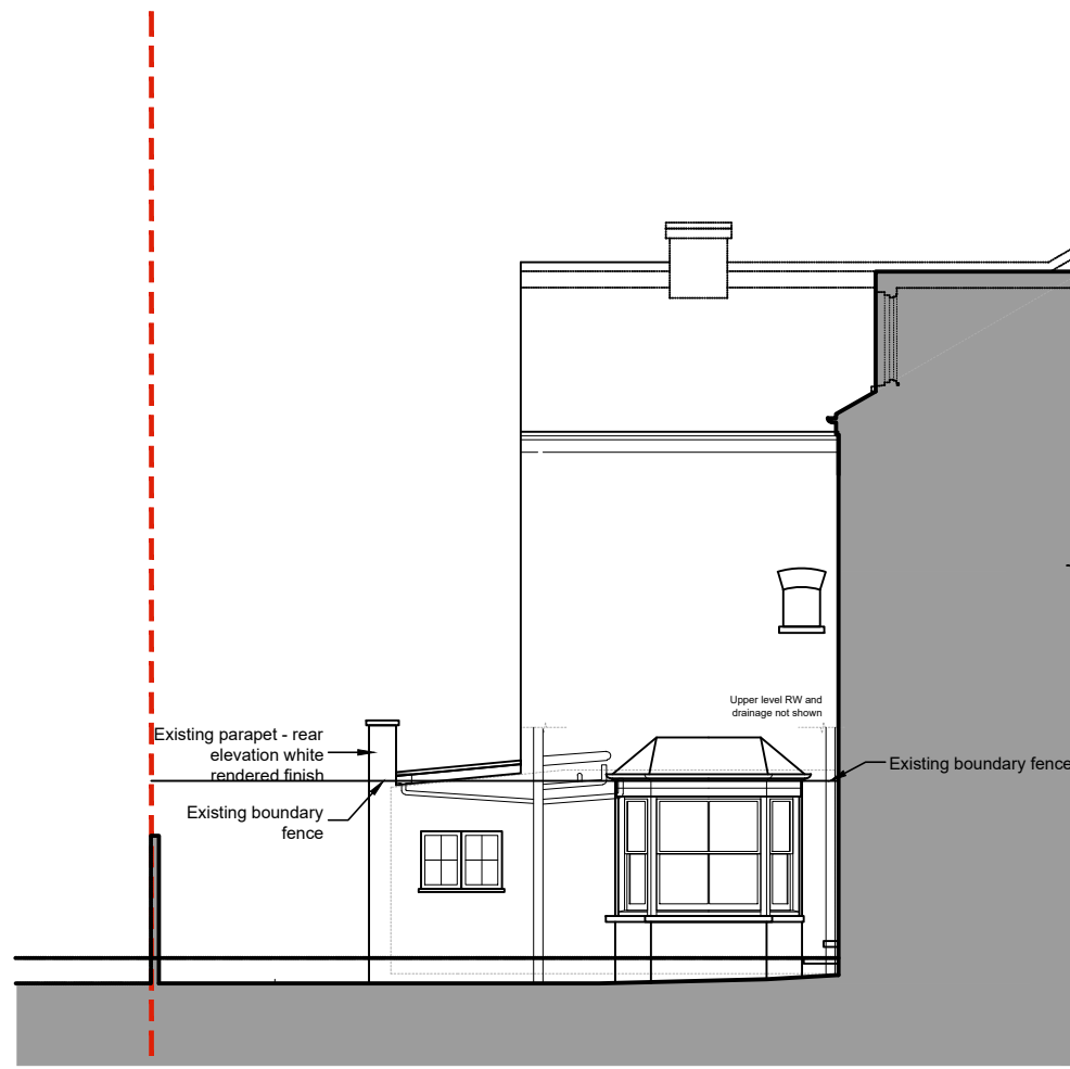
Side elevation
