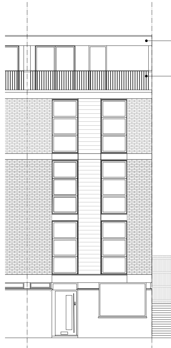
(01)250.01 Front Elevation
