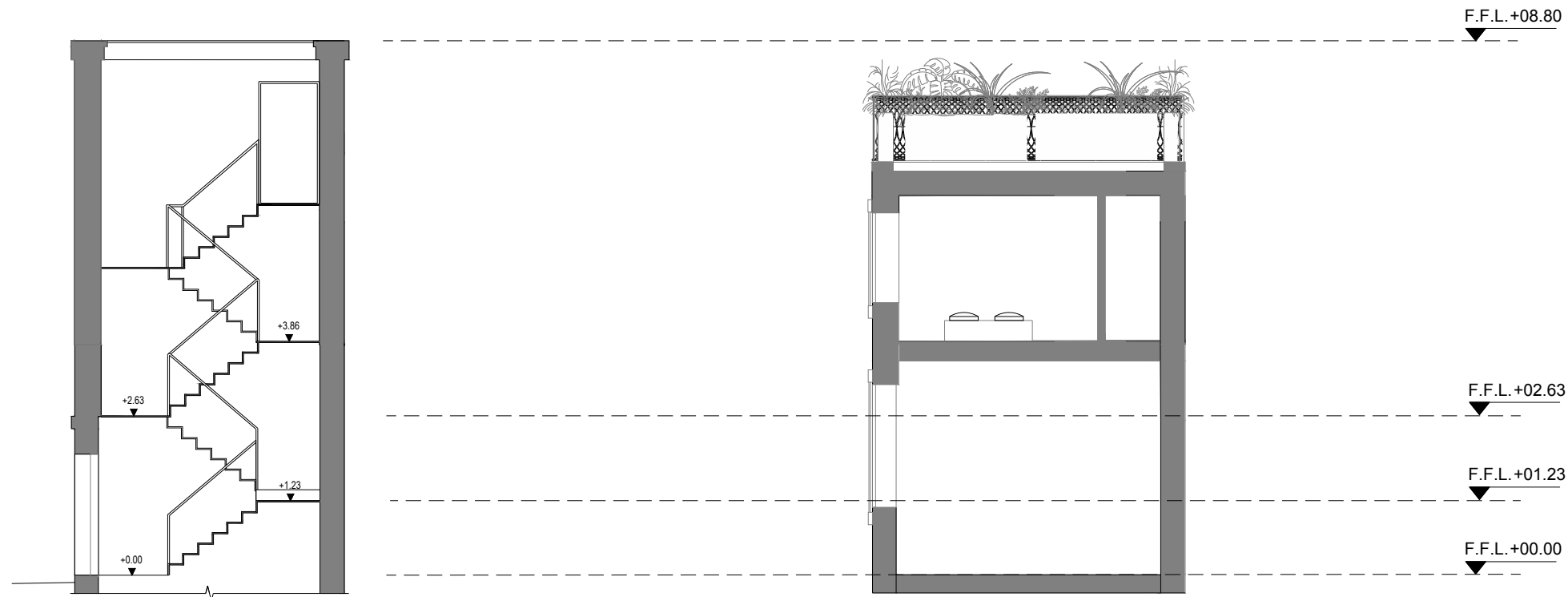
2 Section BB
