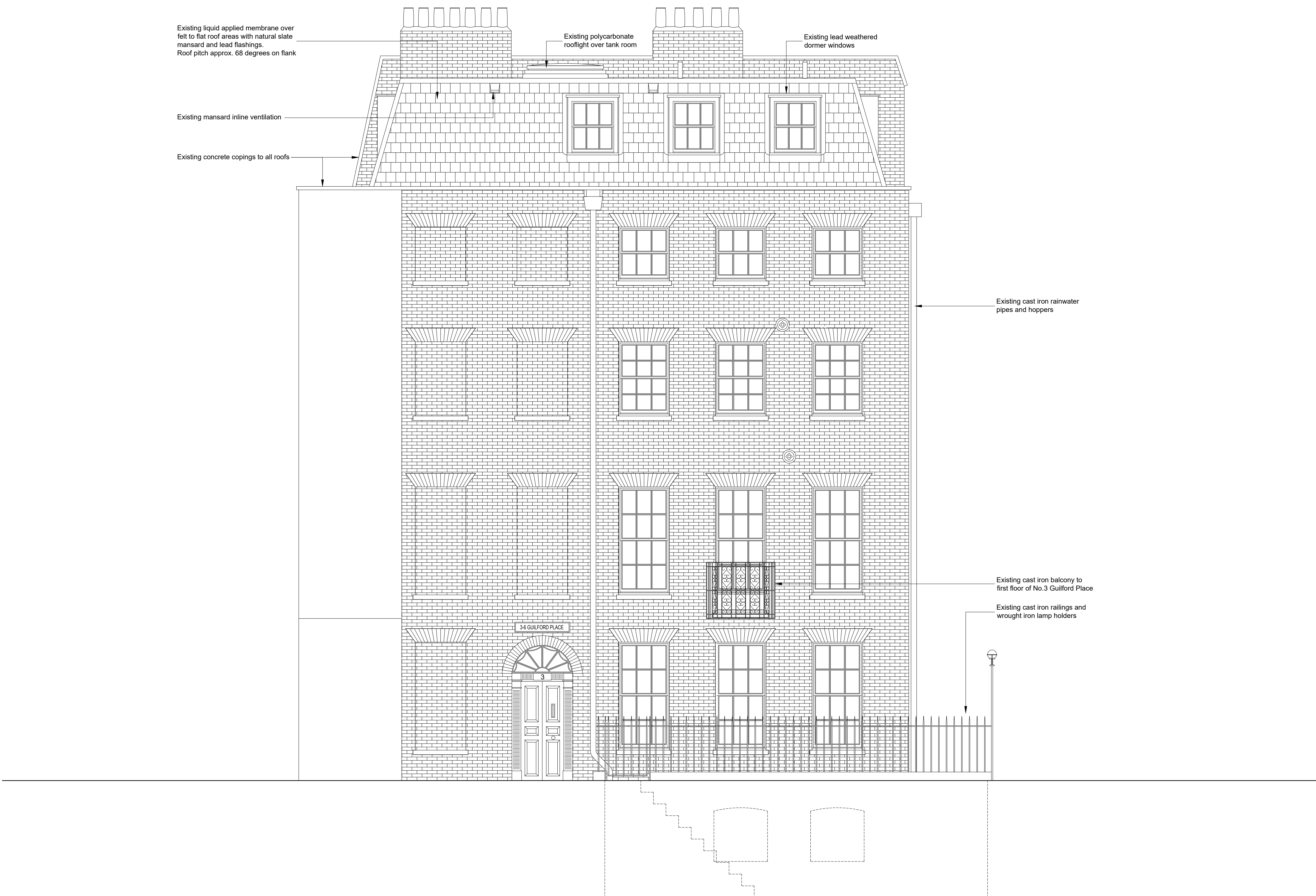
EXISTING SIDE ELEVATION
