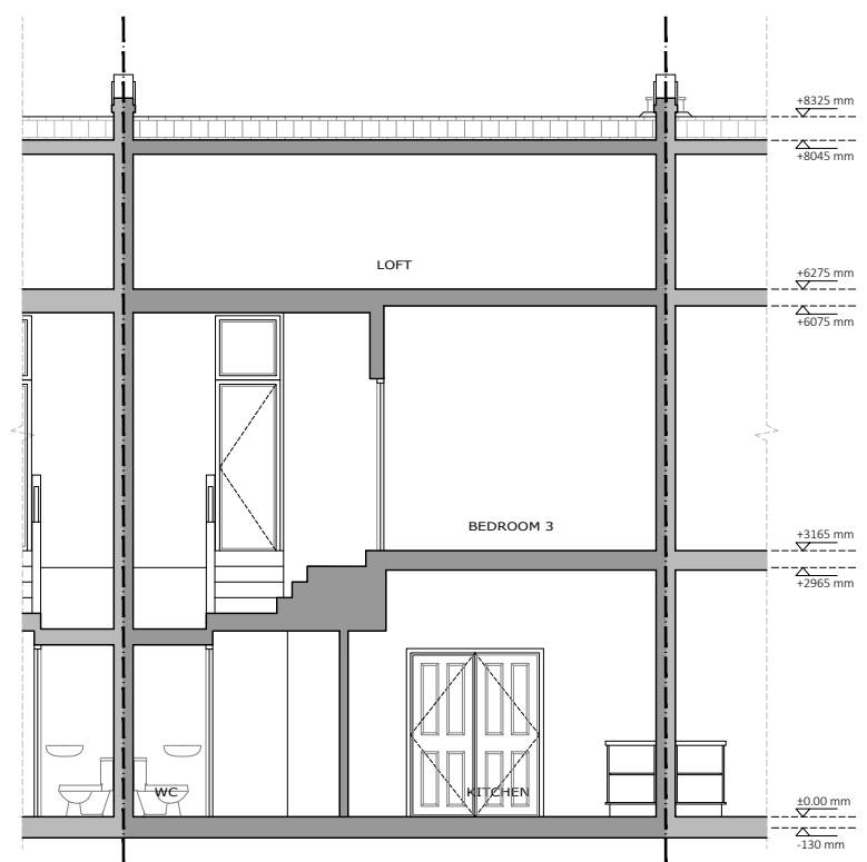
EXISTING SECTION CC
