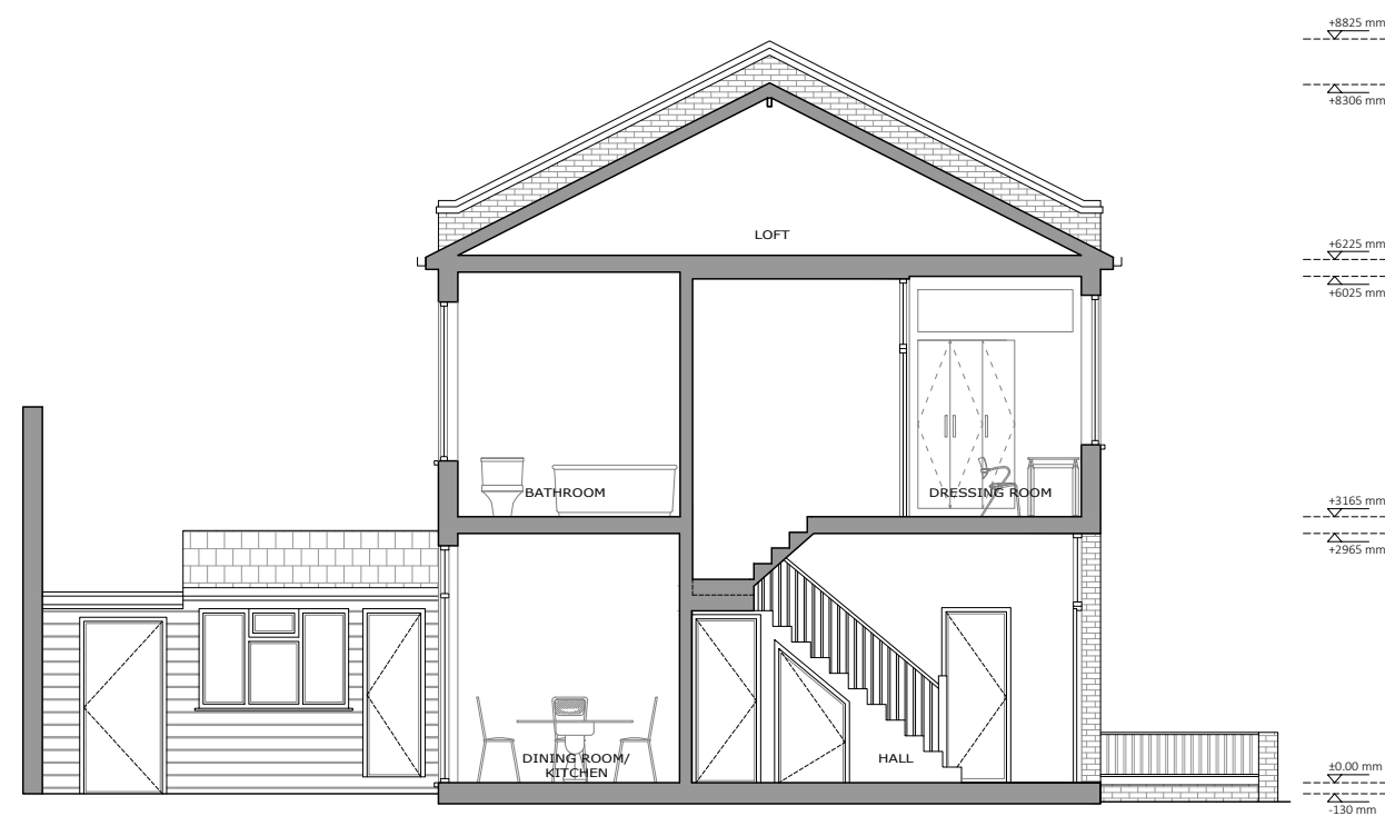
PROPOSED SECTION BB
