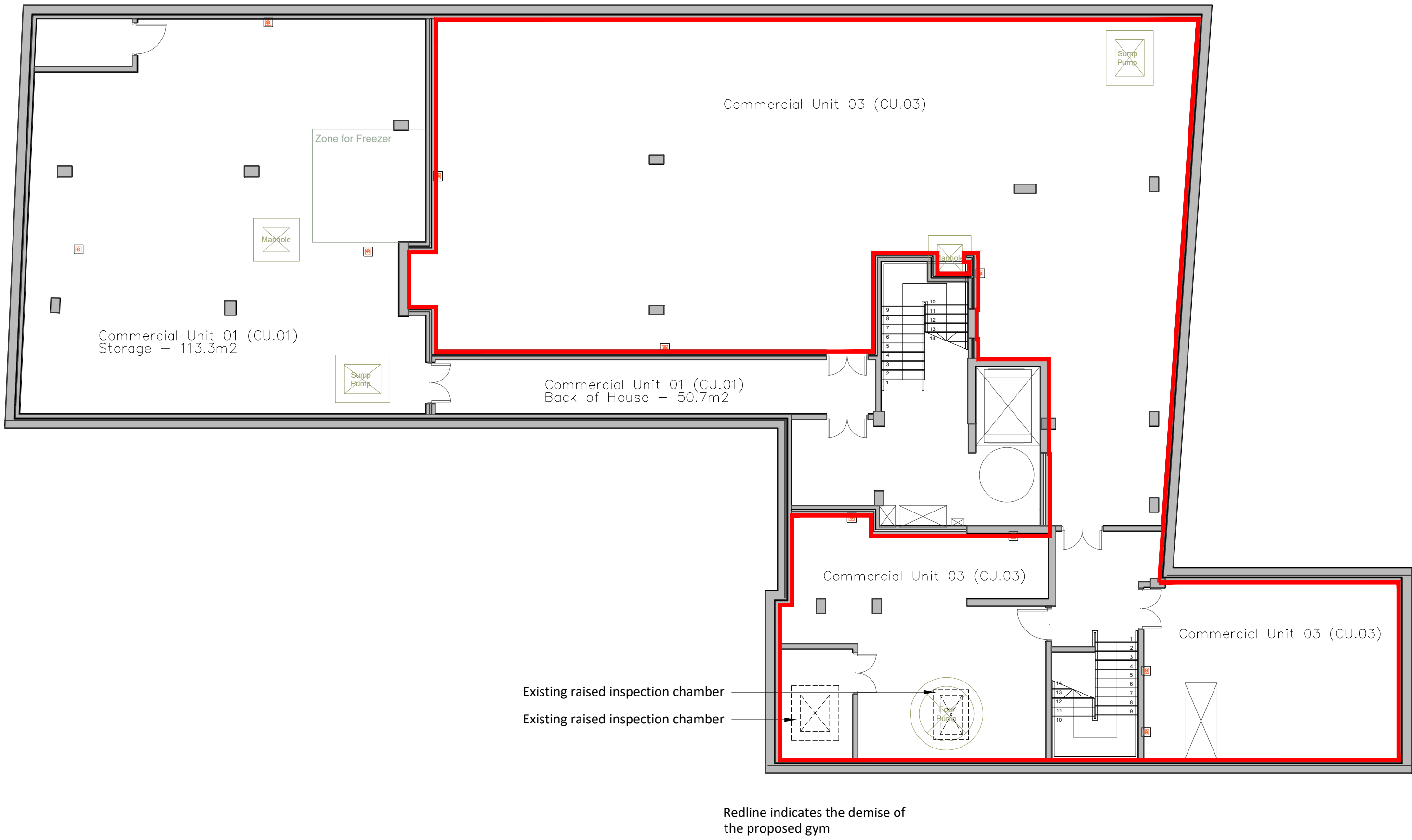
1 | EXISTING BASEMENT FLOOR PLAN SCALE 1:100
