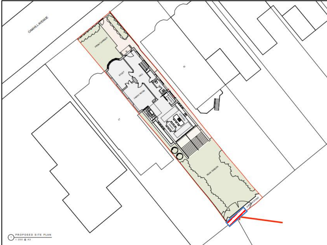
Figure 2.3 Proposed plant unit installation location (Drawing Source: TFF Architects)
