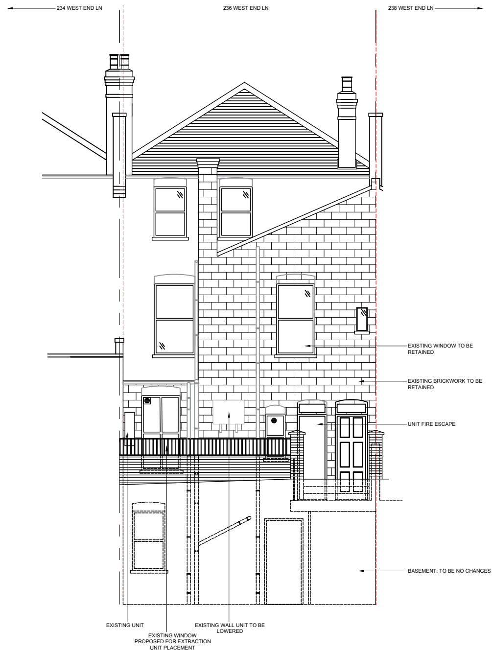
01 REAR EXISTING EXTERNAL ELEVATION 1:100 @ A3
