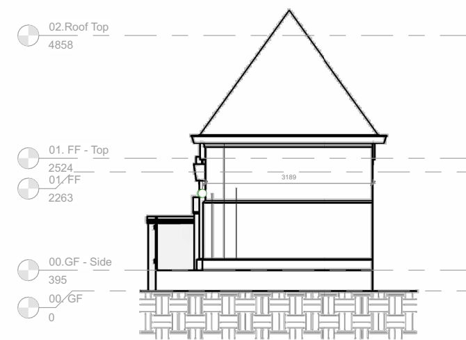
Proposed North View 1 : 50
