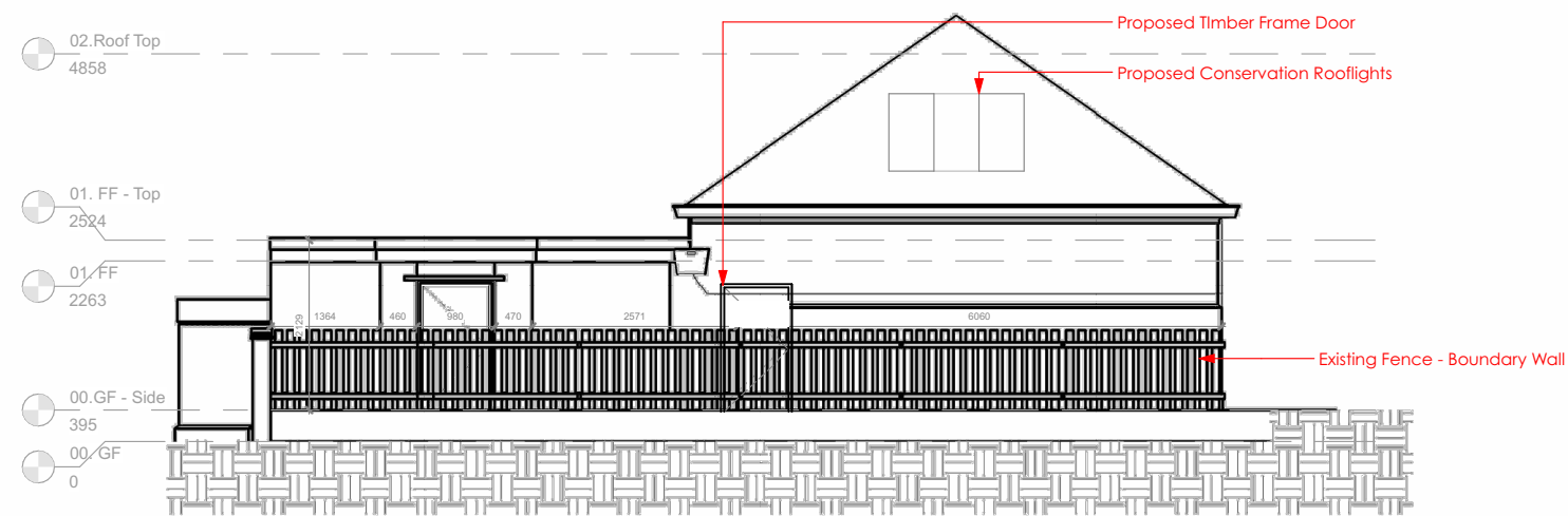
Proposed East View 1 : 50
