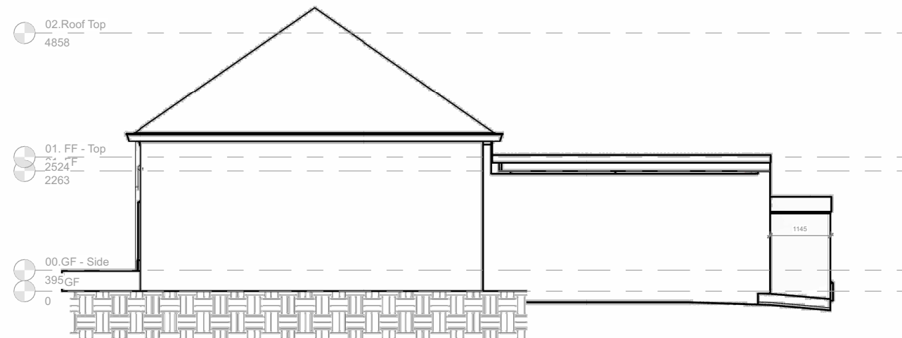
Proposed West View 1 : 50
