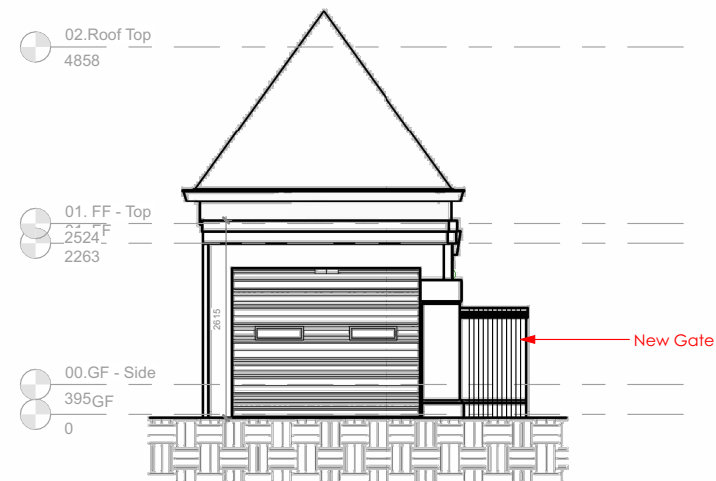
Proposed South View 1 : 50
