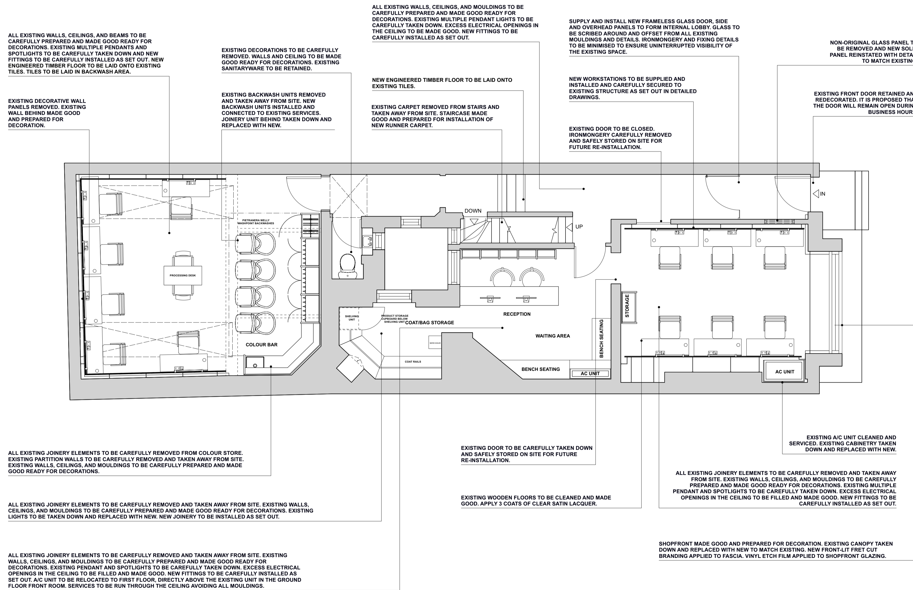
PROPOSED GROUND FLOOR GA
