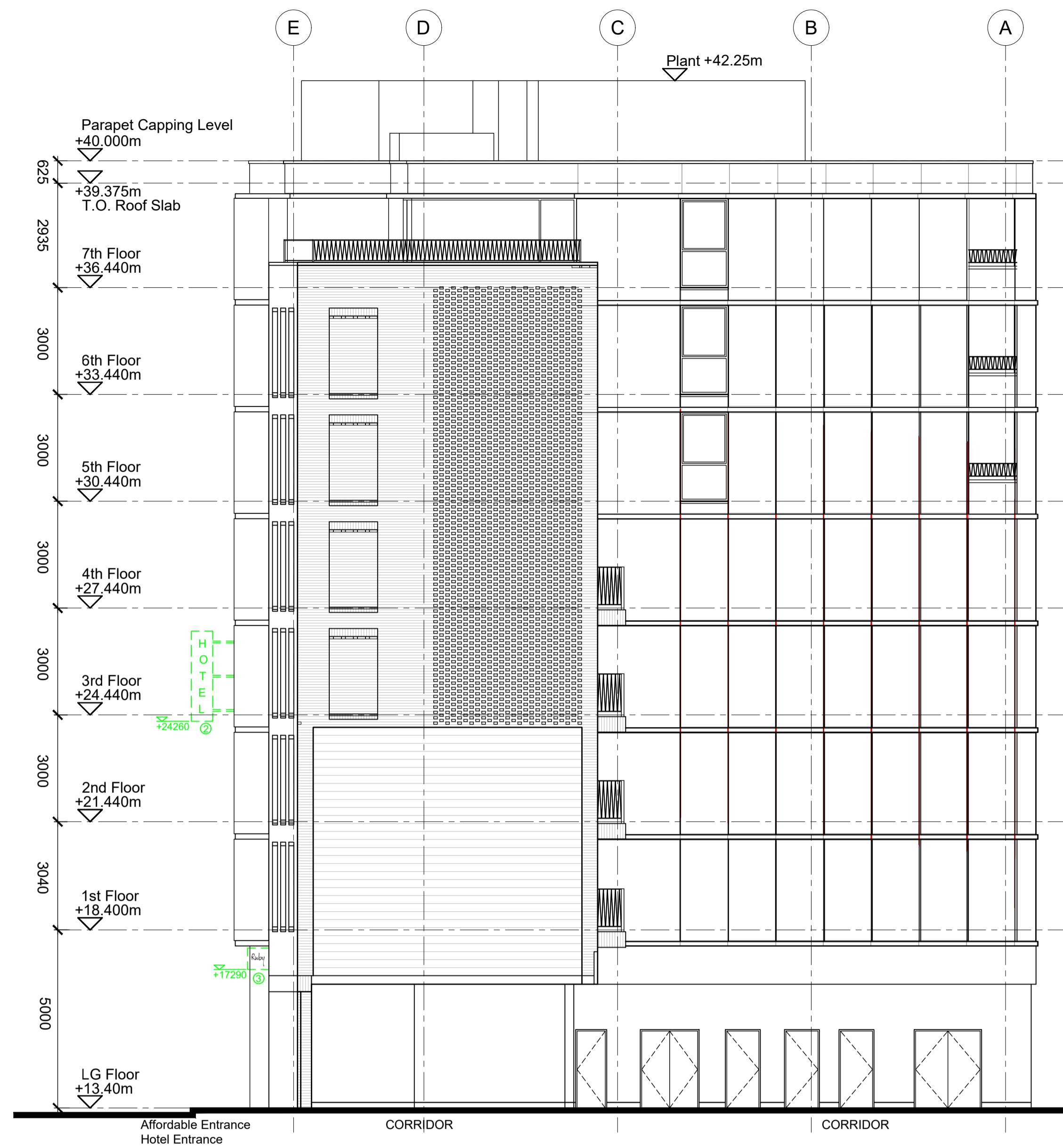
NORTH ELEVATION
