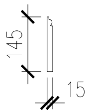
03 PROPOSED SKIRTING PROFILE - SKIRT3
