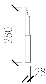
01 PROPOSED SKIRTING PROFILE - SKIRT1
