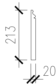
02 PROPOSED SKIRTING PROFILE - SKIRT2
