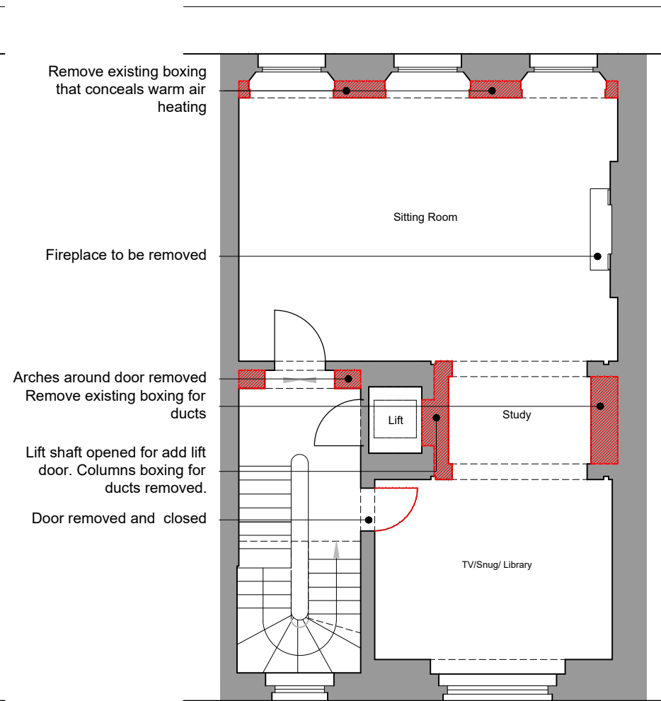
2 Demolition First Floor Plan GHV 1:100 @ A3
