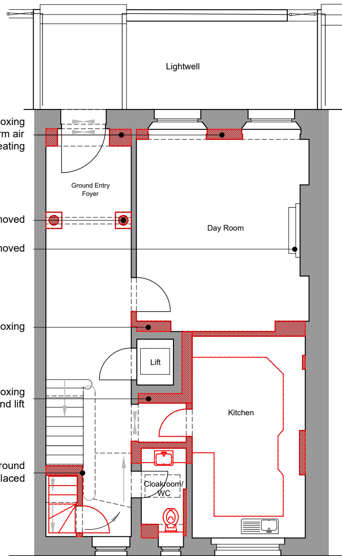
2 Demolition Ground Floor Plan GHV 1:100 @ A3
