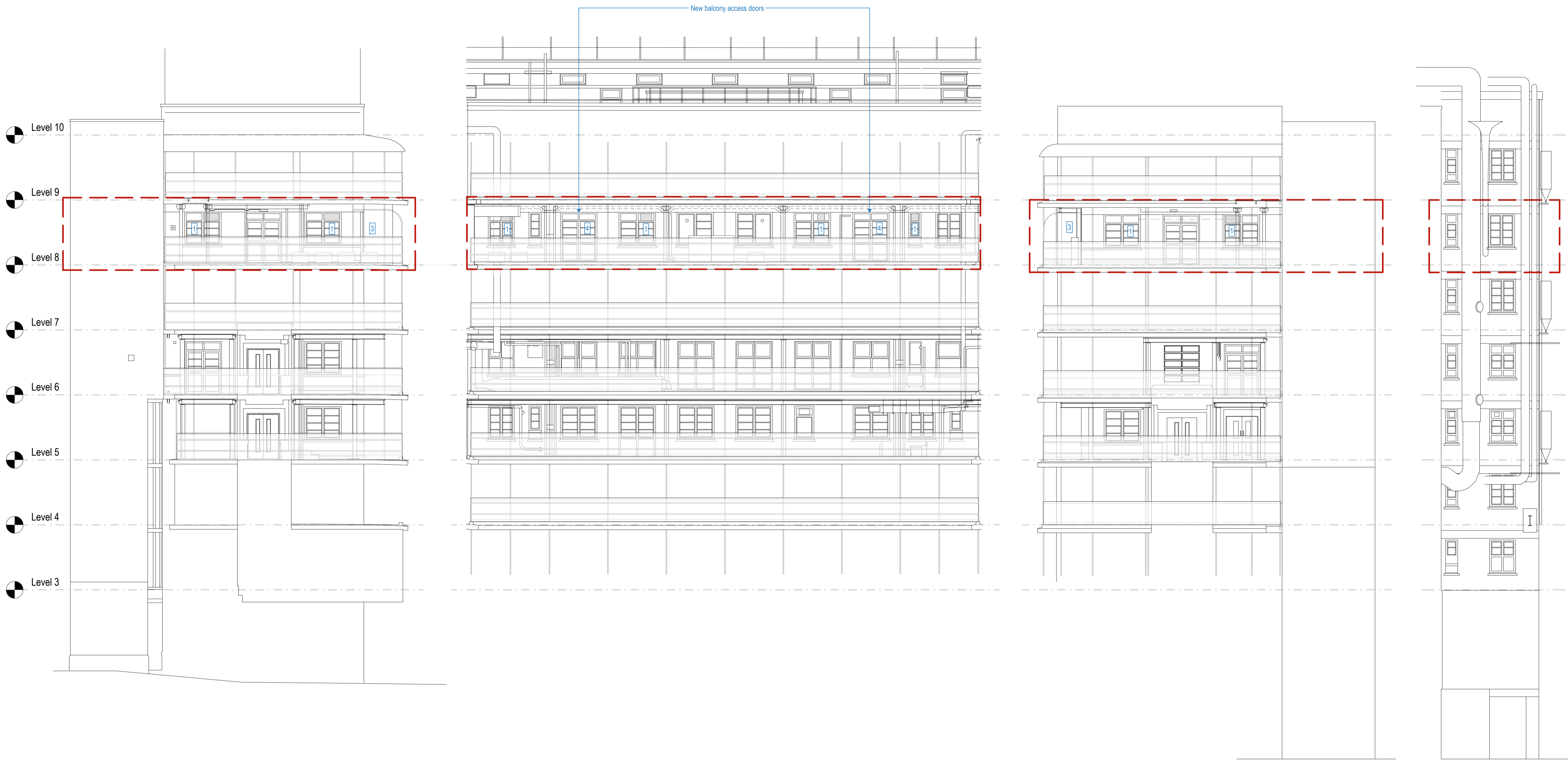
1 3254 South Elevation 8 1 : 100
