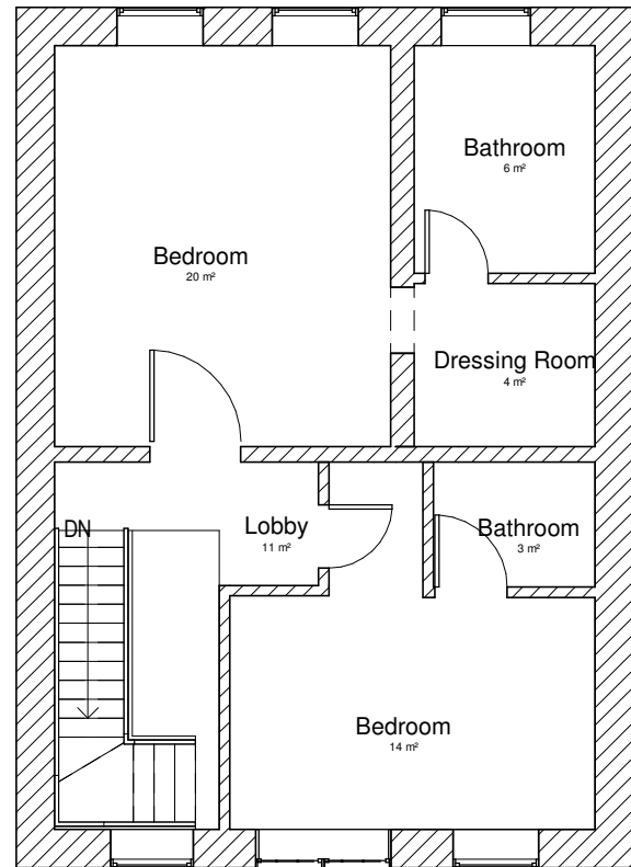
1 Existing First Floor Plan 1 : 100
