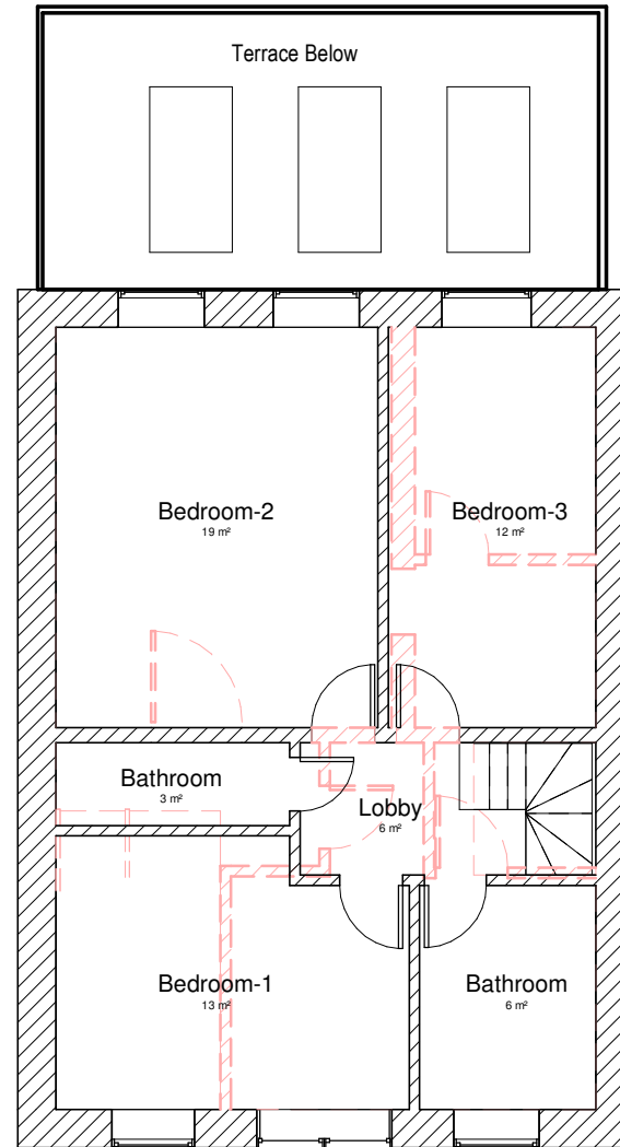
2 Demolish First Floor Plan 1 : 100
