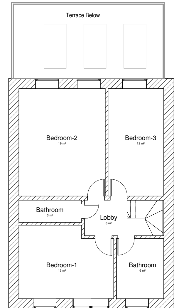
3 Proposed First Floor Plan 1 : 100
