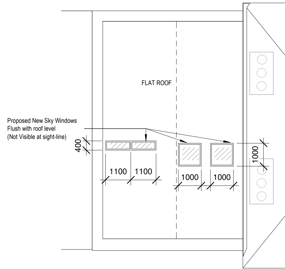
2 Proposed Roof Level 1 : 100
