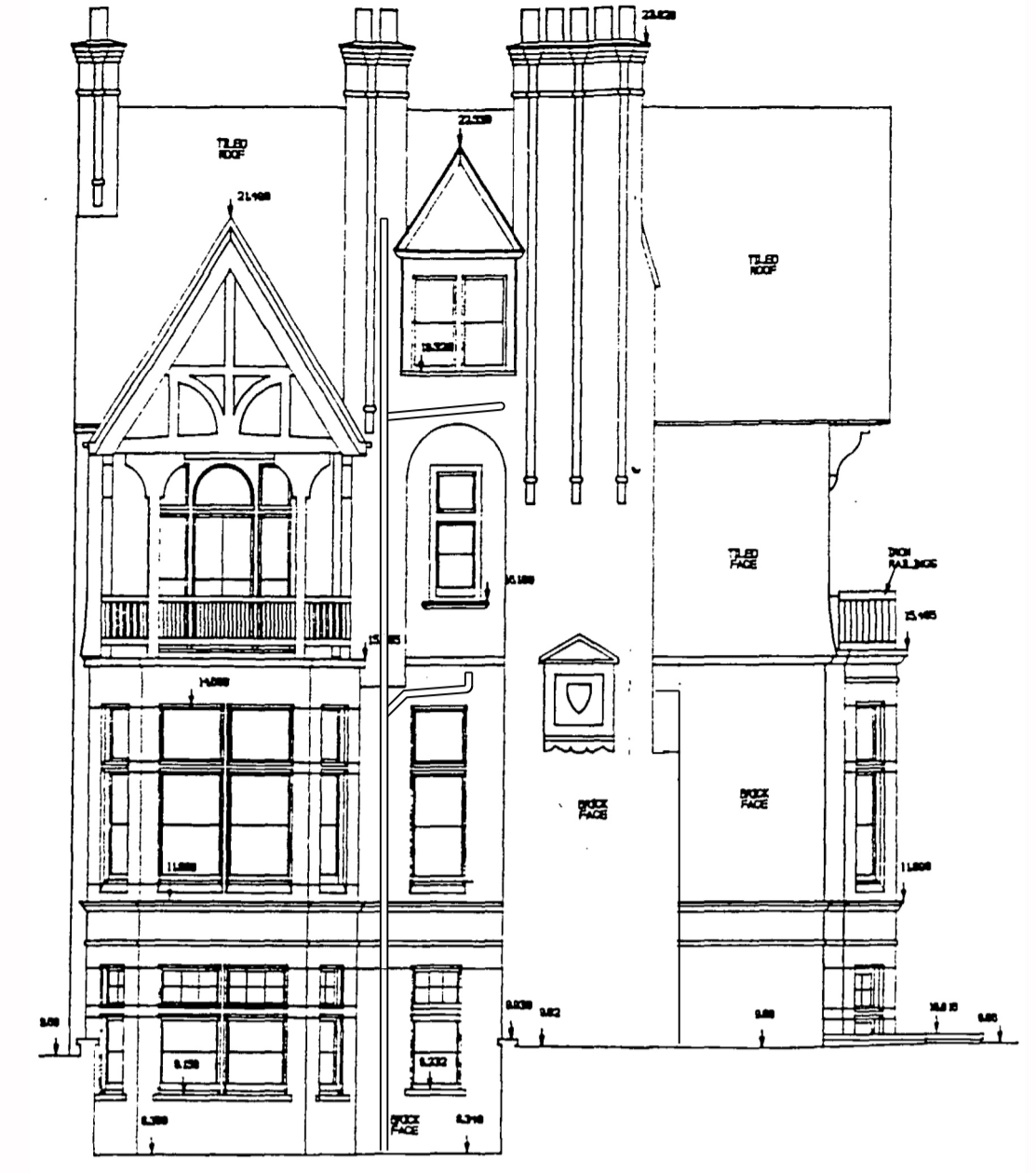
NORTH EAST ELEVATION 1:100
