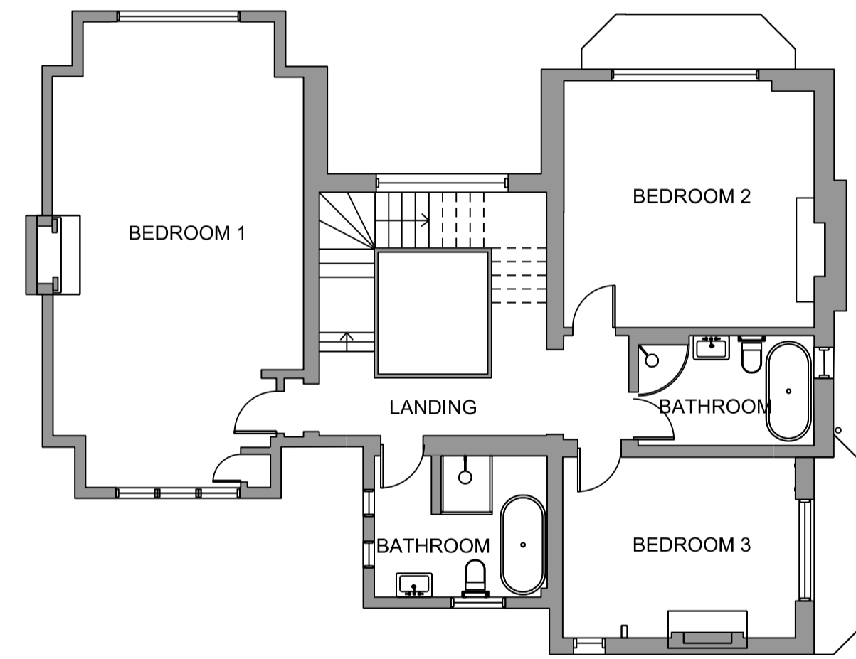
FIRST FLOOR EXISTING 1:100
