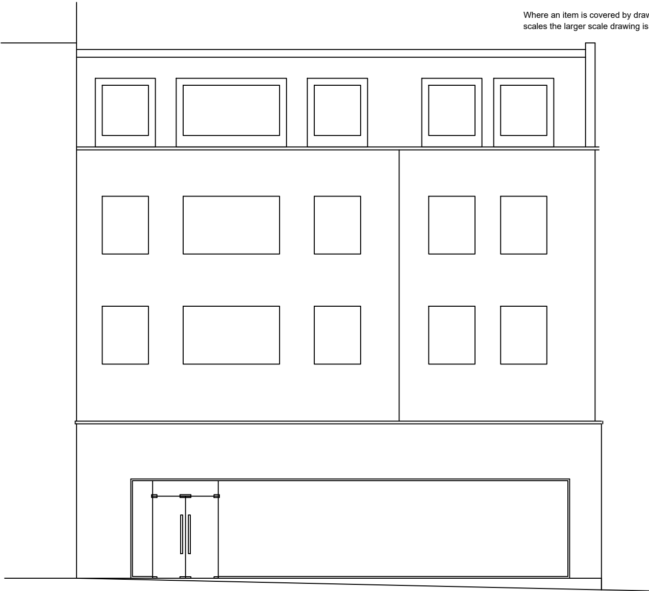
Front Elevation Prior to installation of signage
